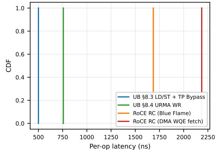
Pointer chase (READ)
