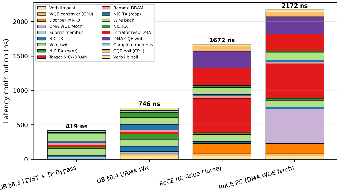
Decomposed latency budget (link=100 ns, 64 B, conc=1, polling)
