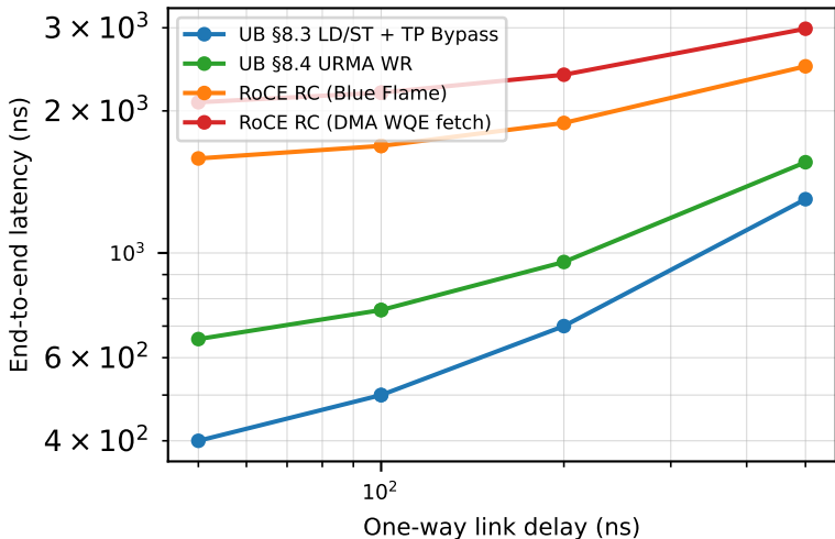
Latency vs link delay (conc=1, payload=64 B)
