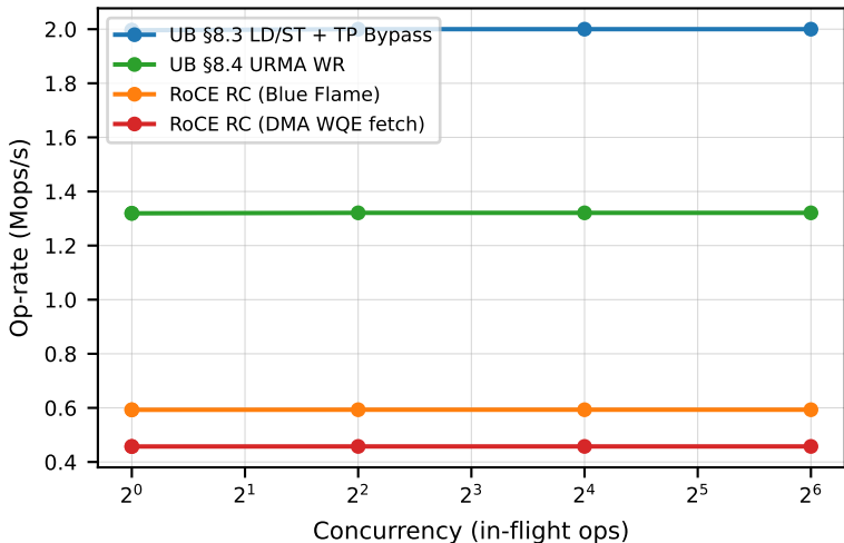
Op-rate vs in-flight depth (link=100 ns, payload=64 B)
