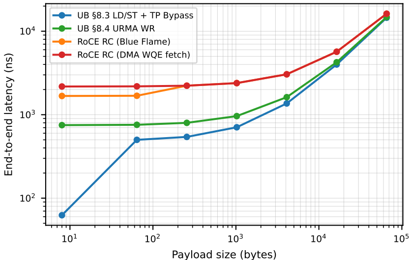
bulk_read: latency vs payload (link=100 ns, conc=1)
