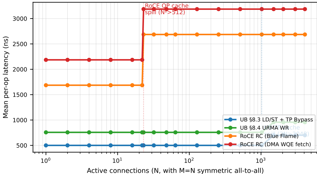
NIC SRAM context-cache spill (READ verb, 64 B, link=100 ns)
