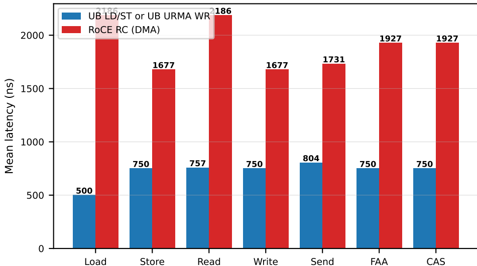
Per-verb latency: UB (LD/ST or URMA WR) vs RoCE DMA (link=100 ns, conc=1)
