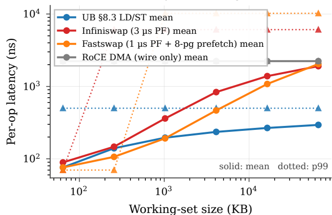
(b) Zipfian latency vs working set ( \alpha=0.99 )
