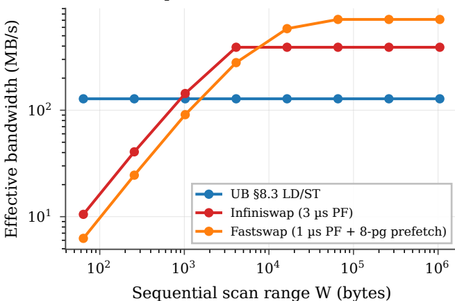
(c) Sequential scan bandwidth vs W
