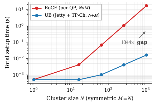
Figure 32: P1.1: total connection-setup time at symmetric N=M . RoCE's O(N \cdot M) vs UB's O(N+M) scaling.
