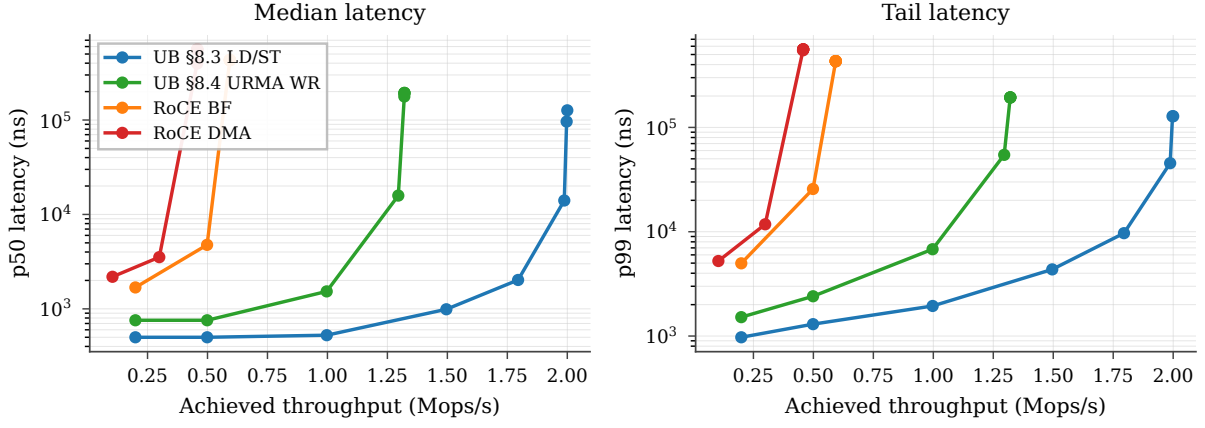
Figure 24: P3.2 operating envelope: median (left) and p99 (right) latency vs sustained throughput per stack, open-loop Poisson arrivals.
