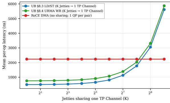
Figure 28: P1.2: UB per-op latency under K-Jetty contention. Linear PSN-allocator scaling; UB still wins until K \approx 255 .
