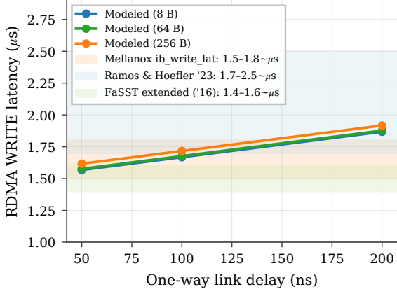
Figure 23: C.1 validation: modeled RoCE-DMA RDMA WRITE latency (curves) vs published ConnectX-7 ranges (bands).
