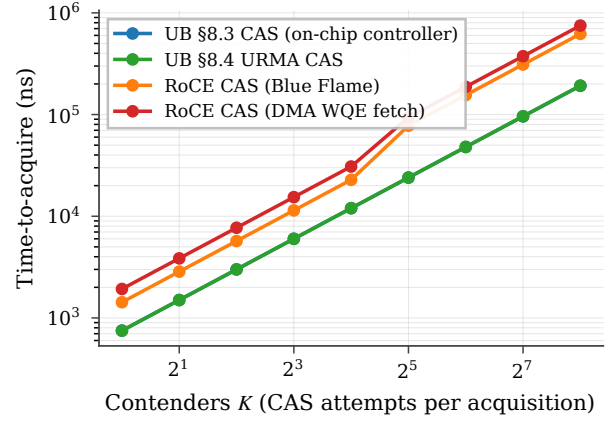
Figure 20: Distributed-lock time-to-acquire vs contender count. Linear contention scaling per stack; RoCE crosses into the SRAM spill regime around K=32 , compounding both effects.
