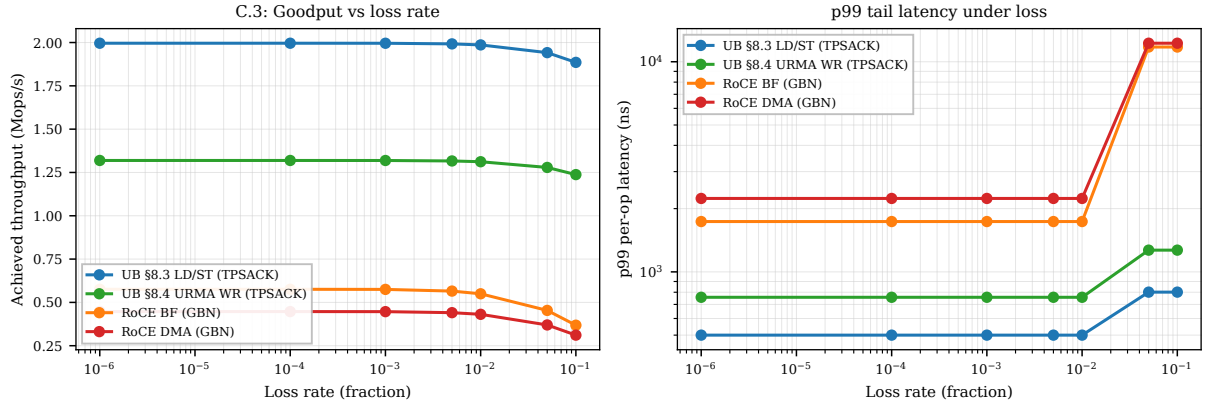
Figure 27: Goodput (left) and p99 tail (right) vs loss rate. Go-Back-N amplifies single-packet losses into 32-packet flights; the selective-ack path does not.
