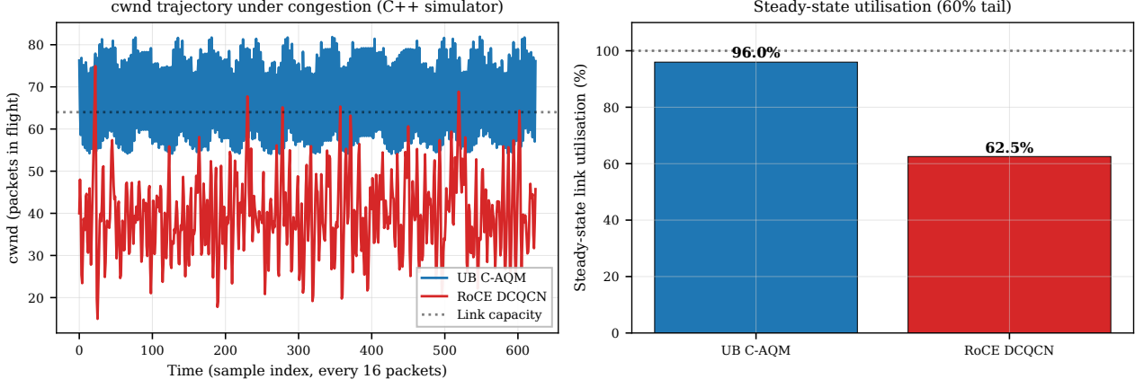
Figure 26: C.2: C-AQM vs DCQCN controller dynamics from the C++ simulator’s CongestionController. cwnd trajectory (left) and steady-state utilisation (right). Parameters are tuned to reproduce published C-AQM behaviour; the spec (§5.3.5.3) leaves the queue-occupancy threshold vendor-defined.
