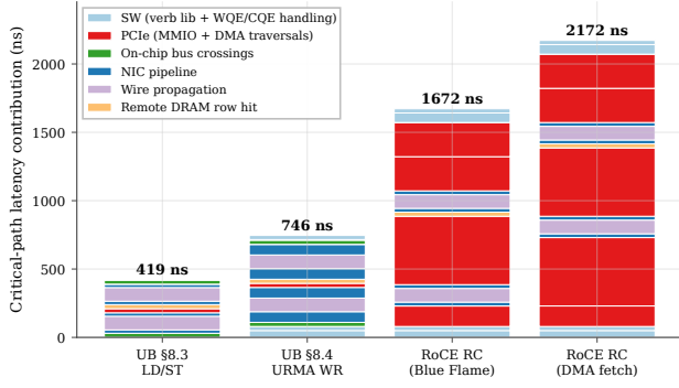
Figure 11: End-to-end latency budget by component, link = 100 ns, payload = 64 B, concurrency = 1.
