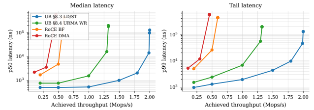
Figure 21: P3.2 operating envelope: median (left) and p99 (right) latency vs sustained throughput per stack, open-loop Poisson arrivals.
