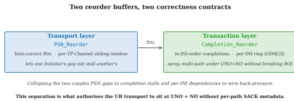
Figure 4: Two reorder buffers serving disjoint contracts: PSN_Reorder delivers byte-correct flits per TP Channel; Completion_Reorder delivers in-INI-order completions per Initiator. The separation is what makes multi-path spraying safe under UNO + NO without per-path SACK metadata.
