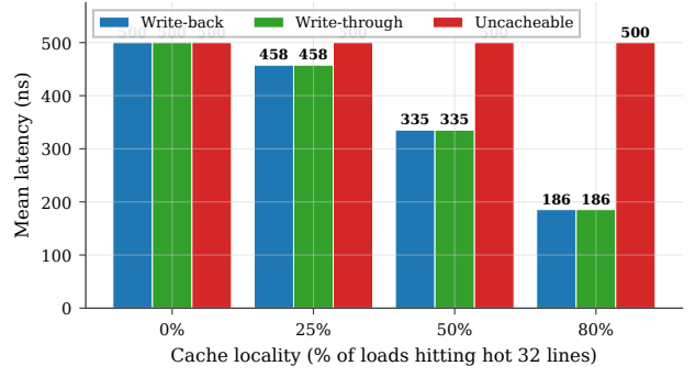
Figure 13: UB §8.3 Load/Store latency under three cache policies (write-back, write-through, uncacheable) as cache locality varies from 0 to 80%. Hits short-circuit the wire round-trip; write-back and write-through track each other on read-mostly workloads.
