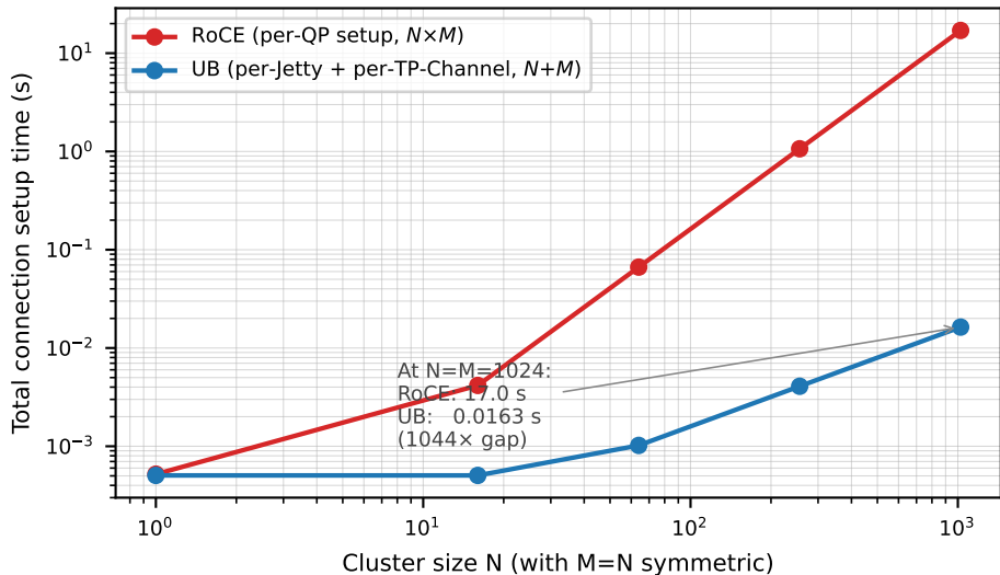
P1.1: connection-setup cost (SystemC, 32 kernel workers)
