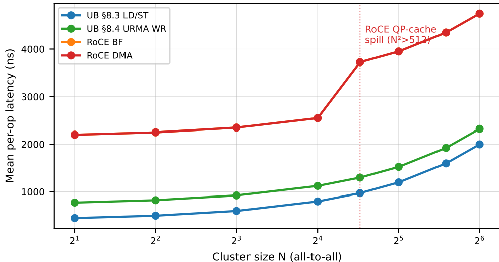
P1.3: SystemC multi-node scaling (N=2..64)
