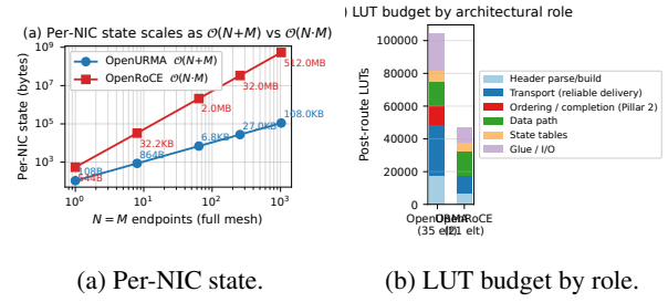
Figure 24: (a) State scaling over (N=M) for OpenURMA’s O(N+M) design vs RoCE’s O(N \cdot M) ; 4,855\times at 1024 endpoints. (b) Post-route LUT budget by architectural role for both stacks.
