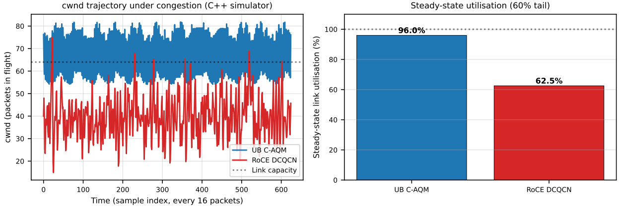
Figure 20: C.2: C-AQM vs DCQCN controller dynamics from the C++ simulator's CongestionController . cwnd trajectory (left) and steady-state utilisation (right).
