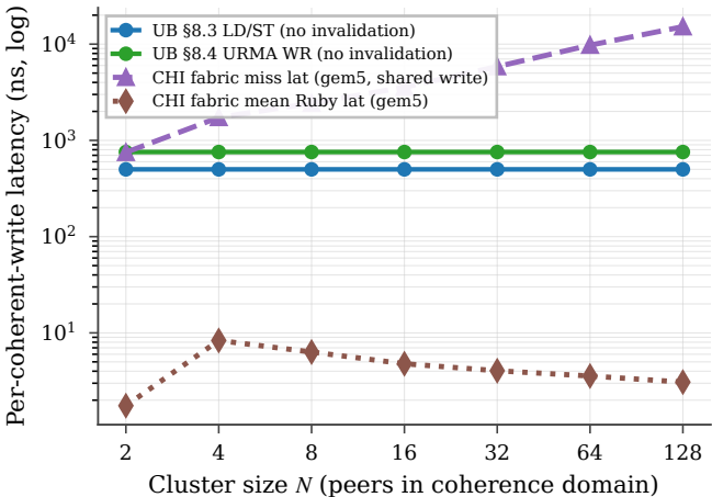
C2: Invalidation broadcast cost (gem5 CHI Ruby)
