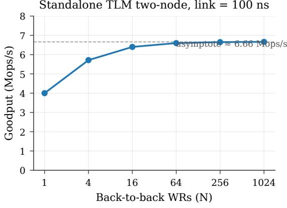
Figure 26: Standalone TLM two-node throughput envelope. Left: goodput vs back-to-back WR count at 100 ns link delay; the curve flattens at \sim 6.66 Mops/s (the 400 ns link-RTT limit). Right: goodput vs per-flit link delay at N=256 (log-log). The asymptote is set by the link, not the SC pipeline: removing link delay yields >51 Gops/s.
