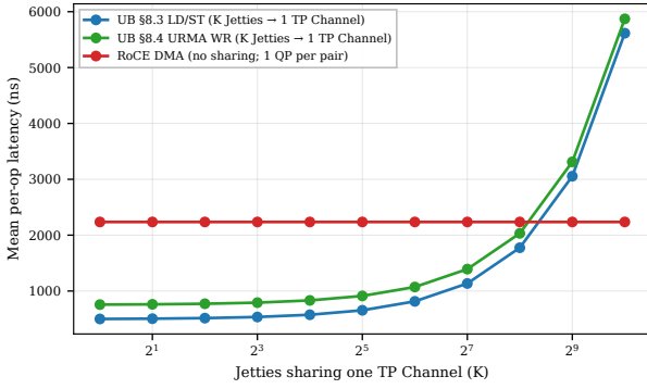
Figure 36: P1.2: UB per-op latency under K-Jetty contention. Linear PSN-allocator scaling; UB still wins until K \approx 255 .
