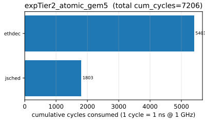
Figure 30: Per-SC-module cycle decomposition emitted by NICTopologySC::emit_decomp_line() during a single_node_fs_clean.py run of the full urma_smoke workload (Phase A/B/L/C). Bars show cumulative “productive” drain sweeps per module after 12608 doorbells, where 1 sweep = 1 ns at the 1 GHz topology clock. ethdec and jsched dominate — the wire-receive decoder and the initiator-side jetty scheduler — consistent with the standalone TLM sim’s per-path cycle attribution (§5).
