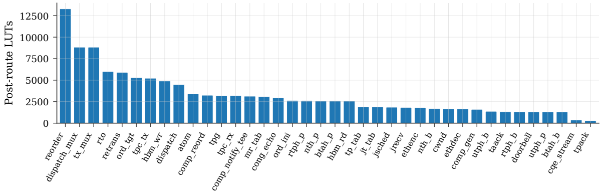
Figure 46: Per-element post-route LUT, sorted descending. All 38 OpenURMA elements meet 322 MHz with positive WNS. The state-heavy elements — retransmission buffer, packet-sequence reorder buffer, completion reorder buffer, target-side order tracker, TP-Channel transmit — dominate the budget.
