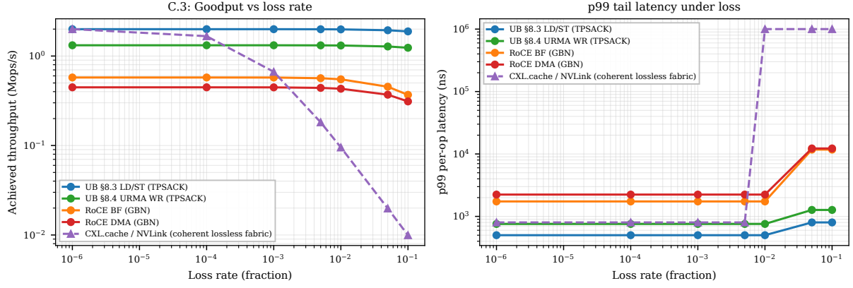
Figure 35: Goodput (left) and p99 tail (right) vs loss rate. Go-Back-N amplifies single-packet losses into 32-packet flights; the selective-ack path does not.
