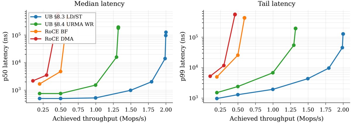
Figure 32: P3.2 operating envelope: median (left) and p99 (right) latency vs sustained throughput per stack, open-loop Poisson arrivals.
