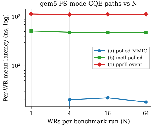
Figure 25: Per-WR mean latency vs N across the three CQE paths. All three paths' per-WR cost is dominated by the per-access overhead component, not amortisable setup; the ioctl floor is \sim 23\times above the MMIO floor and the ppoll floor is another \sim 2.3\times above ioctl .
