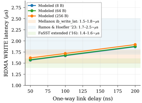
Figure 31: C.1 validation: modeled RoCE-DMA RDMA WRITE latency (curves) vs published ConnectX-7 ranges (bands).
