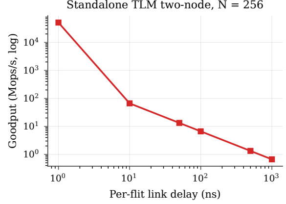
Figure 26: Standalone TLM two-node throughput envelope. Left: goodput vs back-to-back WR count at 100 ns link delay; the curve flattens at \sim 6.66 Mops/s (the 400 ns link-RTT limit). Right: goodput vs per-flit link delay at N=256 (log-log). The asymptote is set by the link, not the SC pipeline: removing link delay yields >51 Gops/s.
