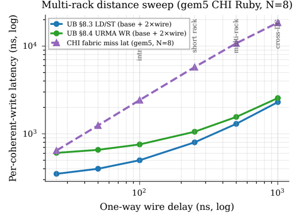
Figure 44: Multi-rack distance sweep: per-coherent-write latency vs one-way wire delay, at fixed cluster size N=8 . CHI cost grows multiplicatively with the wire (snoop RTT compounds across N-1 sharers); UB cost grows additively (one wire RTT). The gap widens monotonically with distance.
