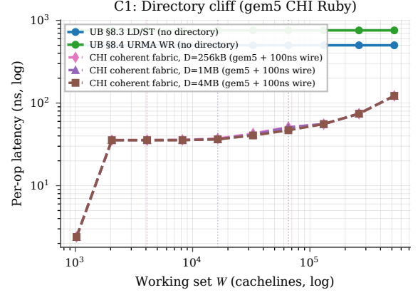
Figure 42: C1: per-op latency vs remote-cached working set W , measured on gem5 CHI Ruby with 100 ns intra-chassis wire delay. Three HNF/directory capacities are swept (256 kB, 1 MB, 4 MB); each curve accelerates sharply once W exceeds the directory size. UB’s two curves are constant in W .
