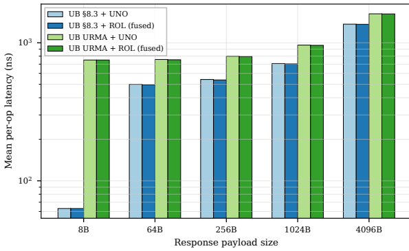
Figure 34: Fused-ack mode vs separate acknowledgement. UB only.
