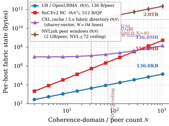
Figure 41: Per-host fabric state vs coherence-domain / peer count N . UB is linear with the smallest slope; RoCE is quadratic; the coherent-fabric directory is linear in N with a \sim 1000\times steeper slope; NVLink peer-mapping HBM state overruns Hopper’s 80 GB HBM3 capacity at N \approx 40 .
