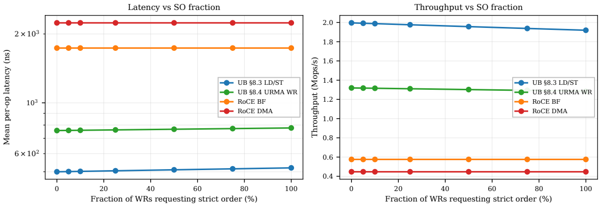
Figure 33: P2.1: latency (left) and throughput (right) vs SO fraction. UB scales linearly with mix; RoCE is flat (always-on strict order).
