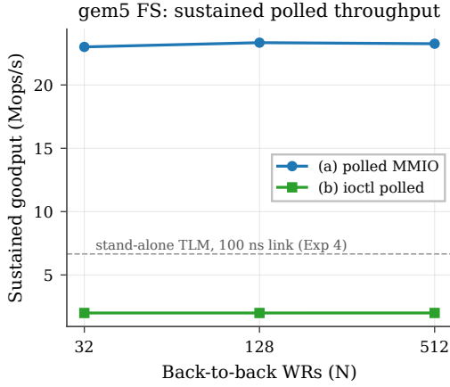
Figure 27: gem5 FS-mode sustained polled goodput vs back-to-back WR count. The polled-MMIO path (a) holds \sim 23 Mops/s; the ioct1 path (b) holds \sim 2 Mops/s. Dashed line marks the standalone-TLM 6.66 Mops/s envelope (link-limited); gem5’s self-loop has zero link delay so the SC pipeline is the bottleneck, not the wire.
