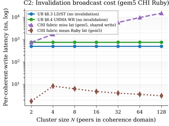
Figure 43: C2: per-coherent-write latency vs cluster size N , measured on gem5 CHI Ruby with 100 ns intra-chassis wire and shared-process pthread workload. CHI miss latency grows from 750 ns at N=2 to 15170 ns at N=128 ( \sim N^{0.65} ), while UB stays flat at 500 ns.
