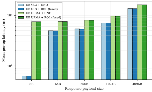
Figure 25: Fused-ack mode vs separate acknowledgement. UB only.
