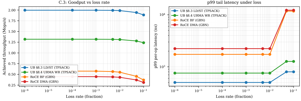
Figure 26: Goodput (left) and p99 tail (right) vs loss rate. Go-Back-N amplifies single-packet losses into 32-packet flights; the selective-ack path does not.
