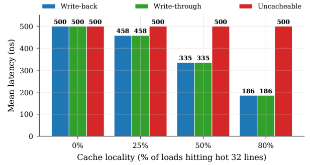
Figure 15: UB §8.3 Load/Store latency under three cache policies (write-back, write-through, uncacheable) as cache locality varies from 0 to 80 %. Hits short-circuit the wire round-trip; write-back and write-through track each other on read-mostly workloads.
