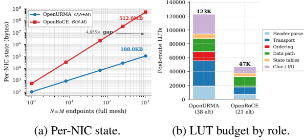
Figure 30: (a) State scaling over (N=M) for OpenURMA’s O(N+M) design vs RoCE’s O(N \cdot M) ; 4,855\times at 1024 endpoints. (b) Post-route LUT budget by architectural role for both stacks.
