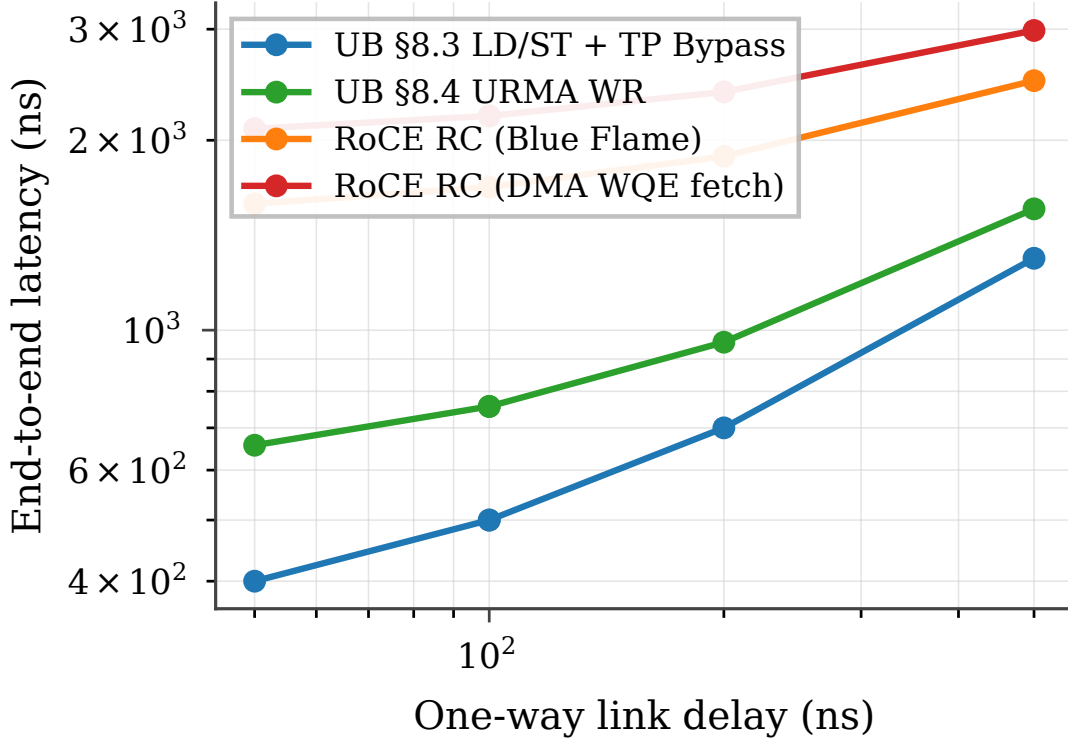
Figure 10: End-to-end latency vs one-way link delay on ptr_chase , concurrency = 1, payload = 64 B.
