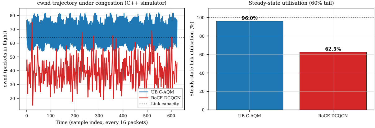
Figure 26: C.2: C-AQM vs DCQCN controller dynamics from the C++ simulator’s CongestionController. cwnd trajectory (left) and steady-state utilisation (right). Parameters are tuned to reproduce published C-AQM behaviour; the spec (§5.3.5.3) leaves the queue-occupancy threshold vendor-defined.
