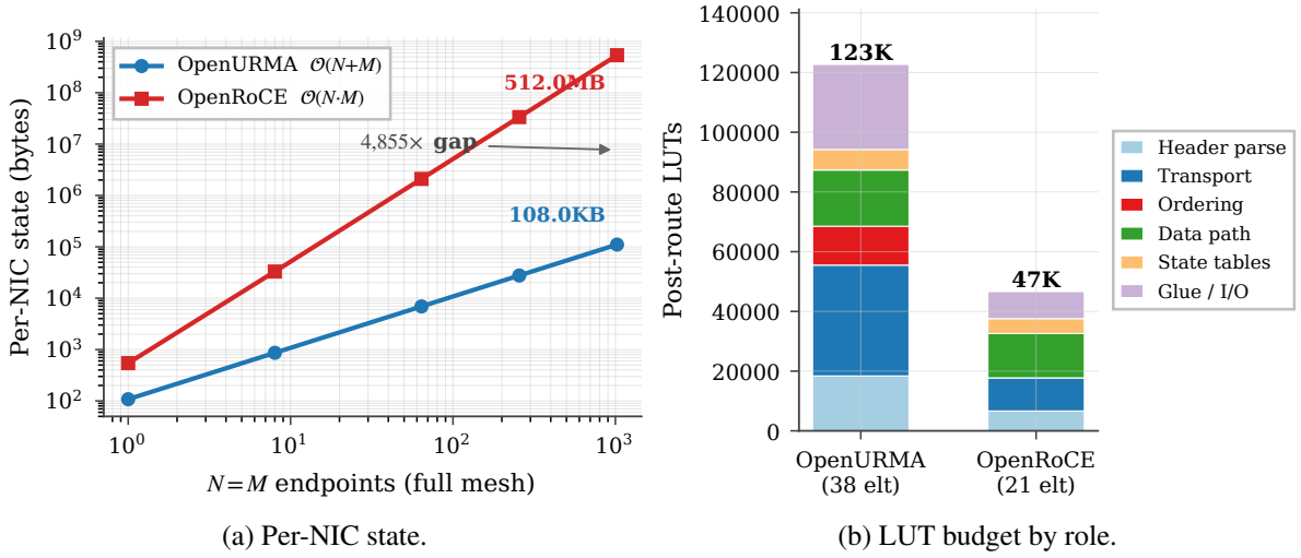
Figure 30: (a) State scaling over ( N=M ) for OpenURMA’s \mathcal{O}(N+M) design vs RoCE’s \mathcal{O}(N \cdot M) ; 4,855\times at 1024 endpoints. (b) Post-route LUT budget by architectural role for both stacks.
