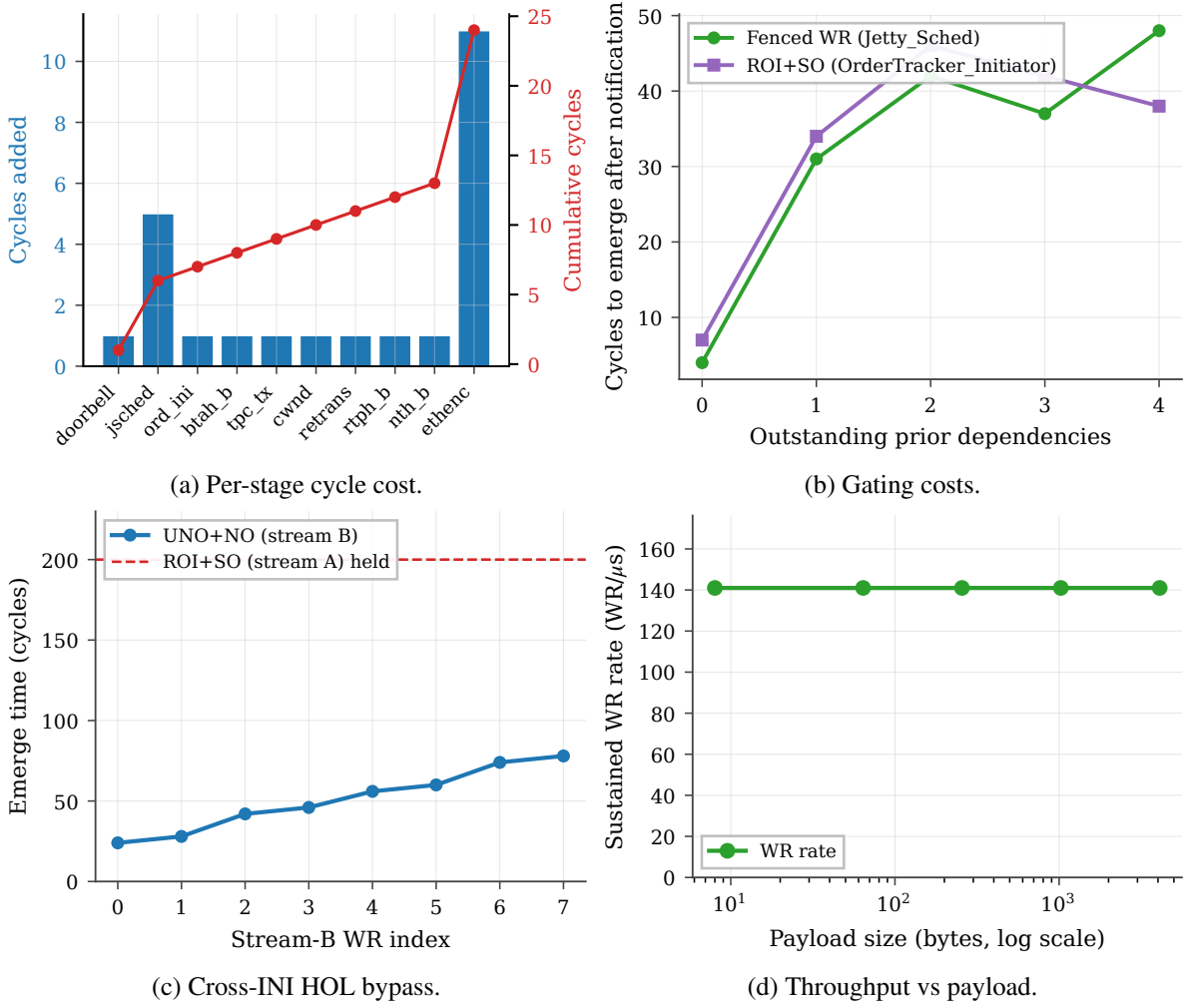
Figure 6: SystemC microbenchmarks. (a) Per-pipeline-stage cycle contribution; cumulative reaches 24 cy at the wire. (b) Cost of Fence and SO gating in cycles after completion notification. (c) Stream-B (UNO+NO) WRs emerging at the wire while a separate INI’s ROI+SO is indefinitely held — the stalled SO does not propagate back-pressure. (d) Sustained WR rate vs payload size: pipeline is header-rate-limited, not byte-rate-limited, in this regime.
