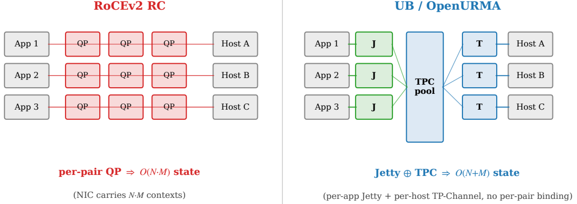
Figure 2: State models compared. RoCE pins one QP to every (application, remote-host) pair; UB decouples per-application state (Jetty) from per-host transport state (TP Channel), and traffic from any Jetty to any host shares a single TP Channel pool with no per-pair binding.
