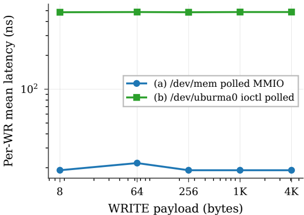
gem5 FS: latency vs payload (N=16)
