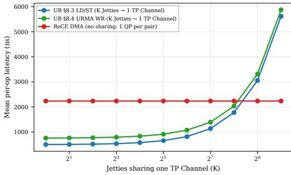
Figure 34: P1.2: UB per-op latency under K-Jetty contention. Linear PSN-allocator scaling; UB still wins until K \approx 255 .
