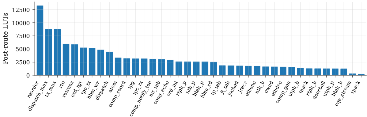
Figure 40: Per-element post-route LUT, sorted descending. All 38 OpenURMA elements meet 322 MHz with positive WNS. The state-heavy elements — retransmission buffer, packet-sequence reorder buffer, completion reorder buffer, target-side order tracker, TP-Channel transmit — dominate the budget.
