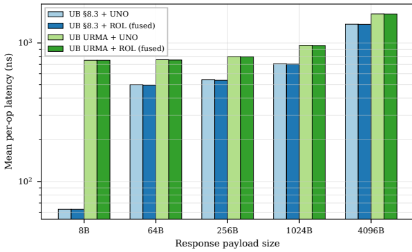
Figure 32: Fused-ack mode vs separate acknowledgement. UB only.
