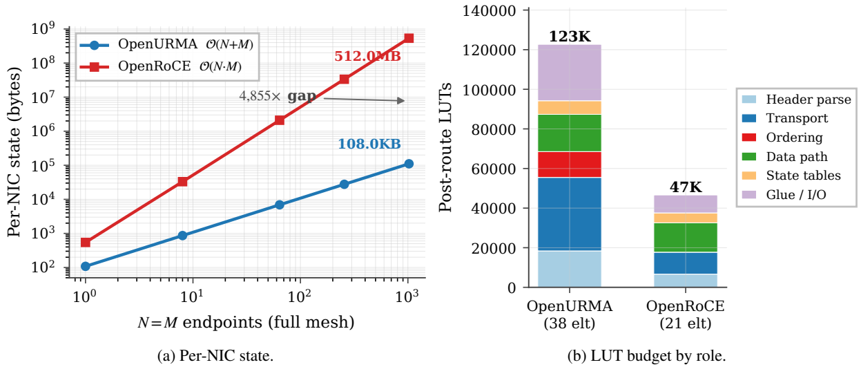
Figure 39: (a) State scaling over (N=M) for OpenURMA’s O(N+M) design vs RoCE’s O(N \cdot M) ; 4,855\times at 1024 endpoints. (b) Post-rte LUT budget by architectural role for both stacks.
