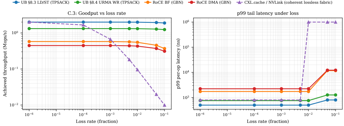
Figure 36: Goodput (left) and p99 tail (right) vs loss rate. Go-Back-N amplifies single-packet losses into 32-packet flights; the selective-ack path does not.
