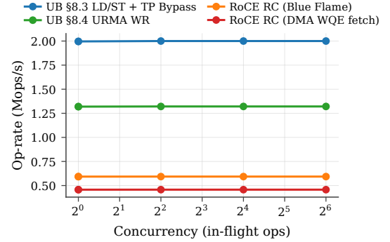
Figure 11: Op-rate vs in-flight depth on pointer-chase, link-delay = 100 ns, payload = 64 B.
