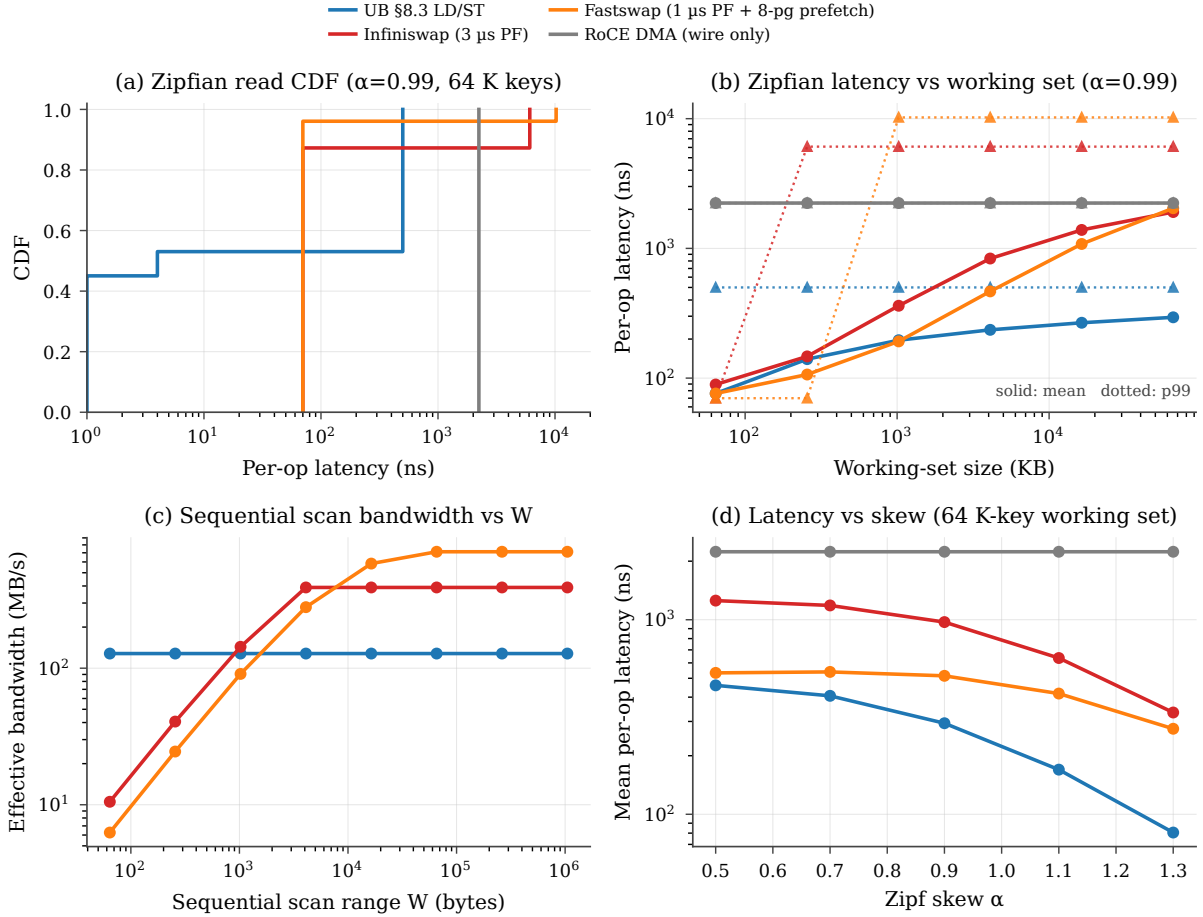
Figure 16: Page-swap baseline comparison. (a) Per-op latency CDF on a 64-K-key Zipfian read workload at \alpha=0.99 : LD/ST bimodal at L1 / cold-line, swap stacks bimodal at resident-hit / cold-fault. (b) Mean + p99 latency vs working-set size: swap stacks track LD/ST below the resident-page cap, diverge above. (c) Sequential scan bandwidth vs W : page-swap amortises 4 KB per fault; LD/ST is one wire round-trip per cache-line in this no-CPU-prefetch model. (d) Mean latency vs Zipf skew \alpha : both bottom out at their respective hit floors as the hot subset narrows.
