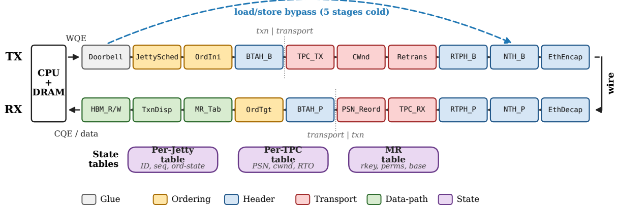
Figure 5: OpenURMA’s NIC as a ClickNP element graph. The TX path (top) flows from CPU doorbell to wire; the RX path (bottom) inverts. Each box is one element, coloured by its functional category (legend at bottom): glue, ordering, header parse/build, transport, on-NIC data path, and state. The dotted vertical markers separate the transaction layer (application-level Jetty scheduling, ordering, memory-region checks, atomic operations, completion generation) from the transport layer (per-host sequencing, retransmission, congestion control). The dashed arc shows the load/store data path (§3.3): a CPU load or store reaches the controller and the bypass element produces a wire packet in five stages cold, skipping the ordering and transport-state machinery entirely.
