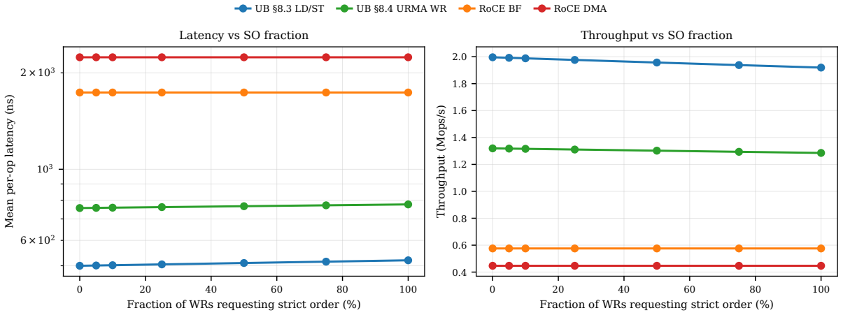
Figure 34: P2.1: latency (left) and throughput (right) vs SO fraction. UB scales linearly with mix; RoCE is flat (always-on strict order).
