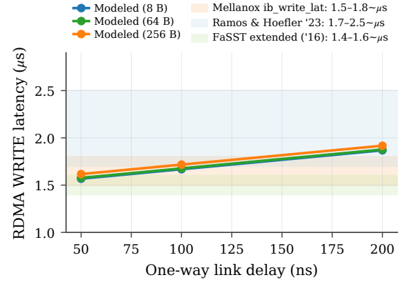
Figure 32: C.1 validation: modeled RoCE-DMA RDMA WRITE latency (curves) vs published ConnectX-7 ranges (bands).
