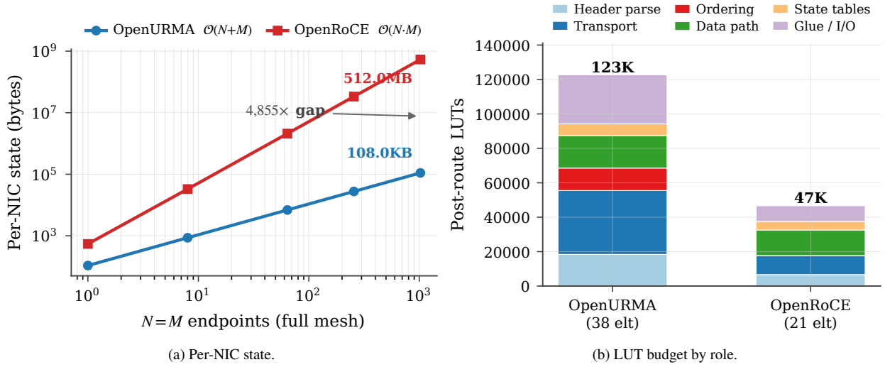
Figure 46: (a) State scaling over (N=M) for OpenURMA’s \mathcal{O}(N+M) design vs RoCE’s \mathcal{O}(N \cdot M) ; 4,855× at 1024 endpoints. (b) Post-route LUT budget by architectural role for both stacks.
