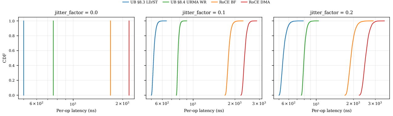
Figure 21: Per-op latency CDFs under jitter. UB’s tail ( p_{99.9}-p_{50} \leq 155 ns) stays an order of magnitude smaller than RoCE’s ( p_{99.9}-p_{50} \geq 660 ns at jitter_factor = 0.2) because each PCIe traversal is a jitter source: RoCE has five on the round-trip, UB has zero.
