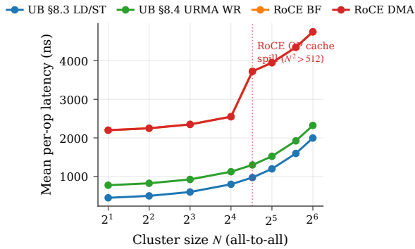
Figure 40: P1.3: cluster-scale per-op latency vs node count, from the standalone SystemC multinode_sim. RoCE crosses the QP-cache spill at N=23.
