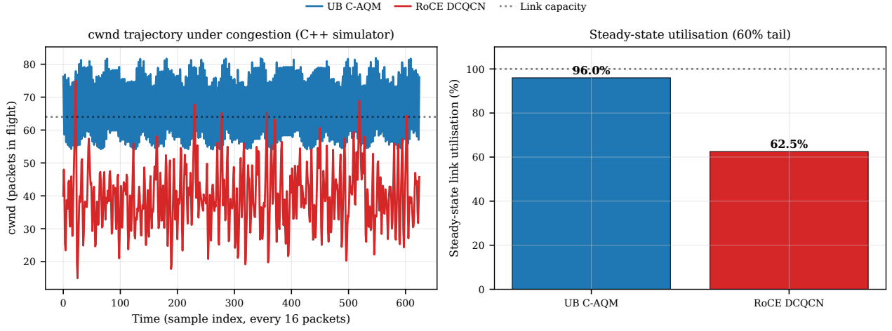
Figure 38: C-AQM vs DCQCN controller dynamics: congestion-window trajectory (left) and steady-state utilisation (right). Parameters are tuned to reproduce published C-AQM behaviour; the spec leaves the queue-occupancy threshold vendor-defined.
