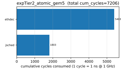
Figure 31: Per-SC-module cycle decomposition emitted by NICTopologySC::emit_decomp_line() during a single_node_fs_clean.py run of the full urma_smoke workload (Phase A/B/L/C). Bars show cumulative “productive” drain sweeps per module after 12608 doorbells, where 1 sweep = 1 ns at the 1 GHz topology clock. ethdec and jsched dominate — the wire-receive decoder and the initiator-side jetty scheduler — consistent with the standalone TLM sim’s per-path cycle attribution (§5).
