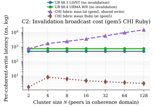
Figure 44: C2: per-coherent-write latency vs cluster size N , measured on gem5 CHI Ruby with 100 ns intra-chassis wire and shared-process pthread workload. CHI miss latency grows from 750 ns at N=2 to 15170 ns at N=128 ( \sim N^{0.65} ), while UB stays flat at 500 ns.
