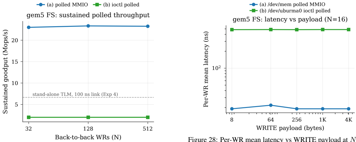
Figure 27: gem5 FS-mode sustained polled goodput vs back-to-back WR count. The polled-MMIO path (a) holds \sim 23 Mops/s; the ioctl path (b) holds \sim 2 Mops/s. Dashed line marks the standalone-TLM 6.66 Mops/s envelope (link-limited); gem5’s self-loop has zero link delay so the SC pipeline is the bottleneck, not the wire.
