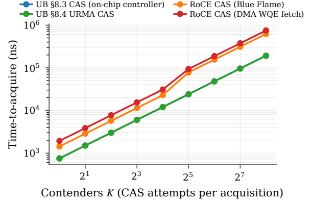
Figure 20: Distributed-lock time-to-acquire vs contender count. Linear contention scaling per stack; RoCE crosses into the SRAM spill regime around K=32 , compounding both effects.
