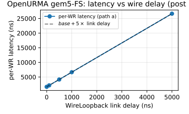
Figure 29: OpenURMA gem5-FS per-WR latency (path-a) polled MMIO) vs WireLoopback link delay, post-Tier-2. With the SC pipeline cycle count and the wire delay folded back into the CPU’s view ( NICTopologySC::pending_wire_delay_ ), per-WR latency tracks base + 5 \times \text{link delay} (1644 ns at 0 ns delay → 26.6 \mu s at 5 \mu s delay): the 5\times slope reflects the wire round-trip (request out, TAACK back) plus the intermediate decoder hops. Before the fix the FS rows were flat at the AtomicCPU instruction floor regardless of delay.
