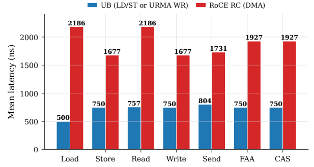
Figure 14: Per-verb mean latency comparison. UB (§8.3 LD/ST for Load/Store; §8.4 URMA WR for Read/Write/Send; §7.4.2.3 atomics for FAA/CAS) vs RoCE RC (DMA WQE fetch). Link = 100 ns, concurrency = 1, payload = 64 B (atomics: 8 B operand).
