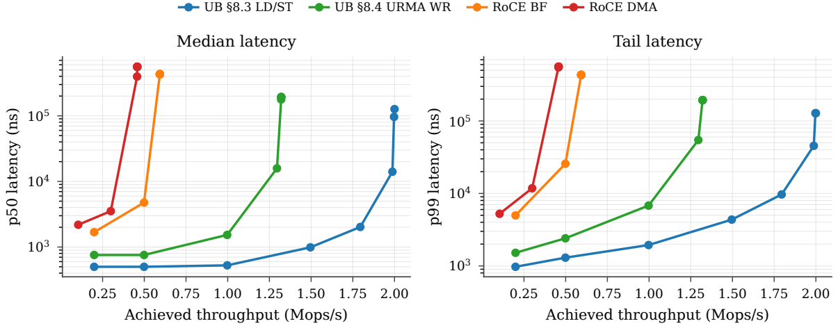
Figure 33: P3.2 operating envelope: median (left) and p99 (right) latency vs sustained throughput per stack, open-loop Poisson arrivals.
