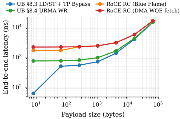
Figure 17: End-to-end latency vs payload size on bulk-read. Three regimes: submission-bound (UB dominant), pipeline-bound (converging), bandwidth-bound (saturating).
