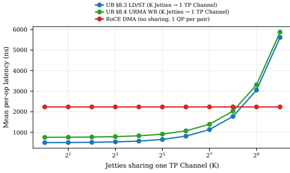
Figure 37: P1.2: UB per-op latency under K-Jetty contention. Linear PSN-allocator scaling; UB still wins until K \approx 255 .
