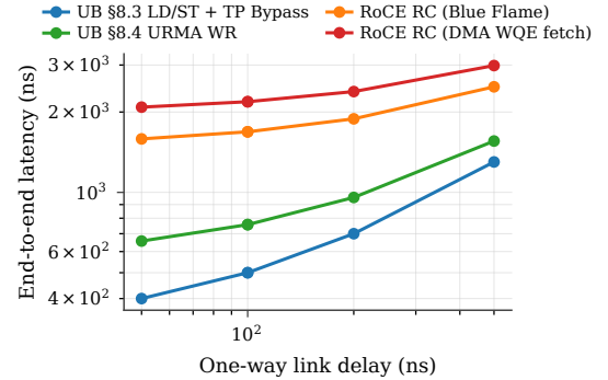
Figure 12: End-to-end latency vs one-way link delay on pointer-chase, concurrency = 1, payload = 64 B.
