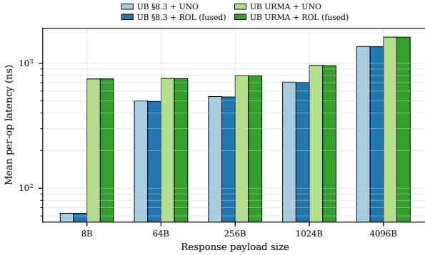
Figure 35: Fused-ack mode vs separate acknowledgement. UB only.
