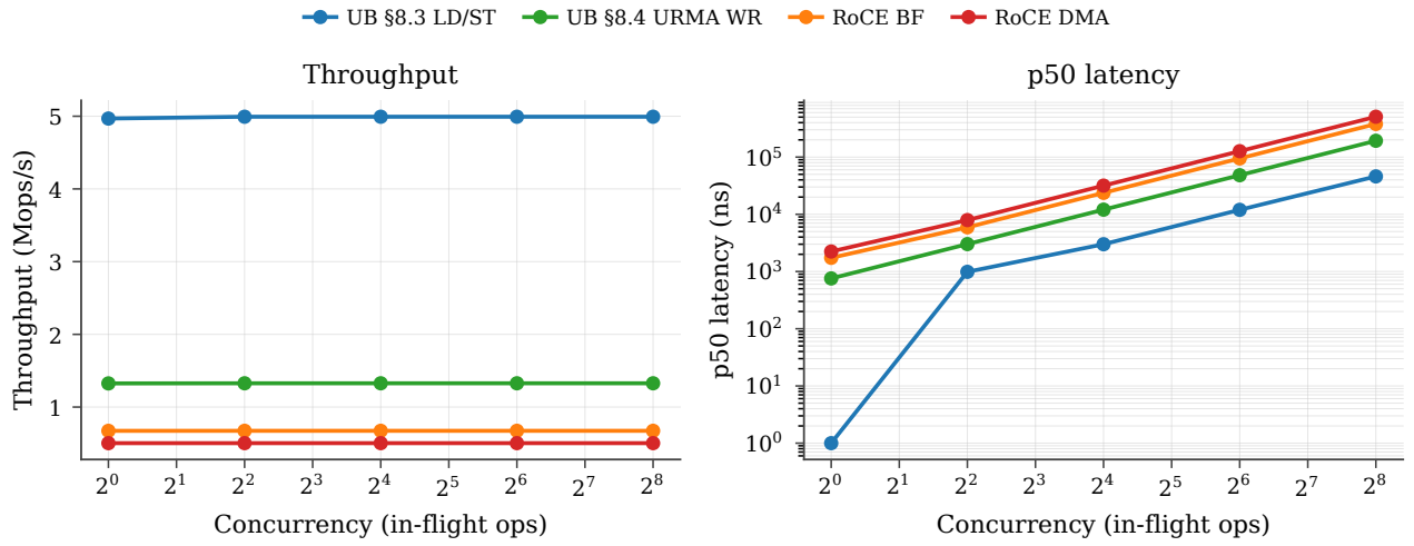
Figure 39: P3.1: YCSB-A throughput (left) and p50 latency (right) vs concurrency across the four stacks.
