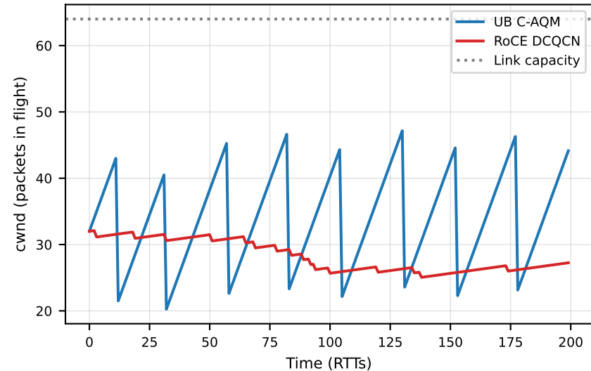
C.2: cwnd trajectory under congestion
