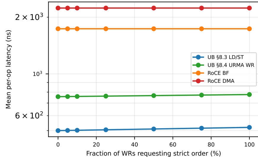
Latency vs SO fraction
