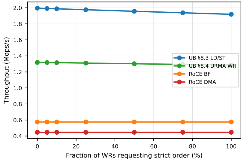
Throughput vs SO fraction
