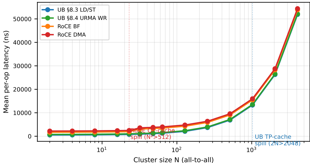
P1.3: cluster-scale latency vs node count
