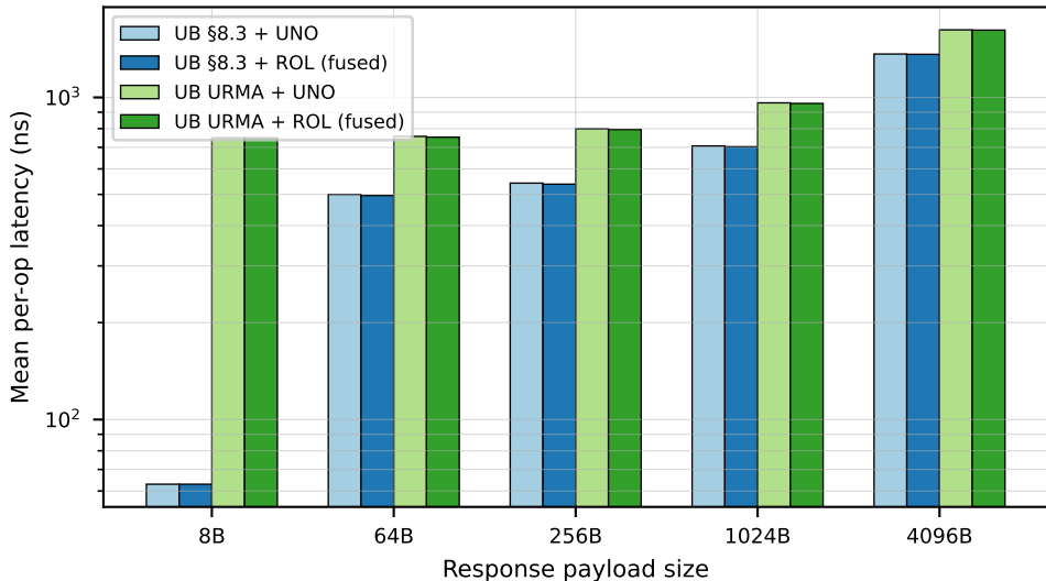
P2.2: ROL fused-ack vs separate TPACK
