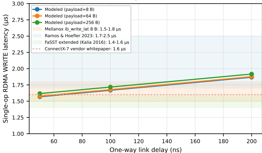
C.1: model validation vs published ConnectX-7 numbers
