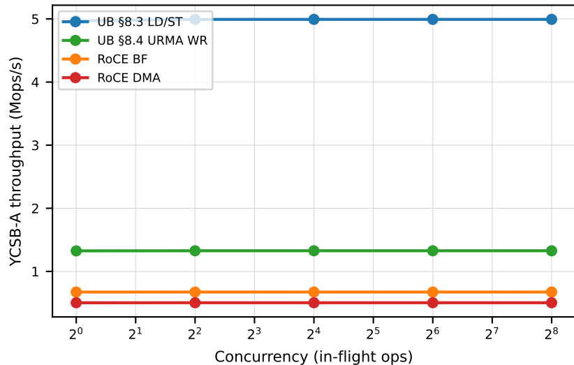
YCSB-A throughput vs concurrency
