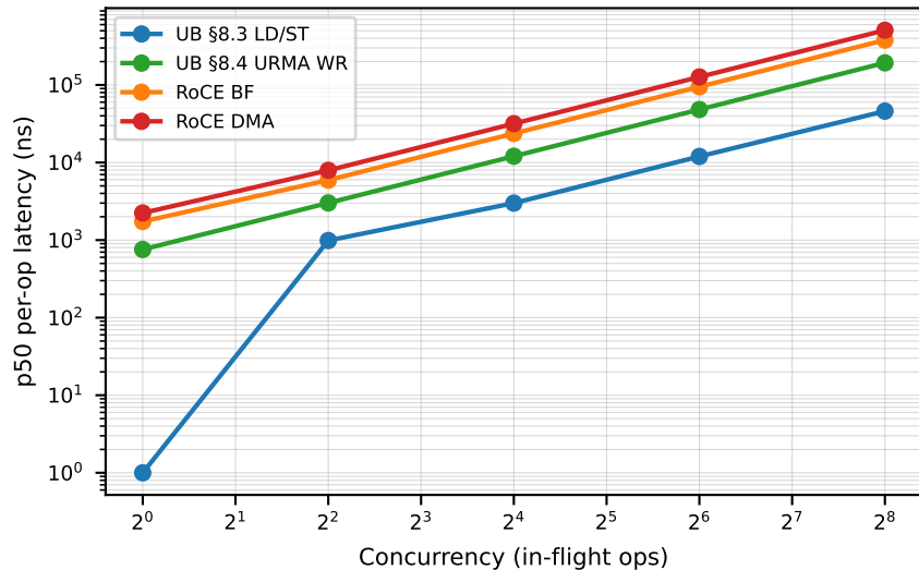
YCSB-A p50 latency vs concurrency
