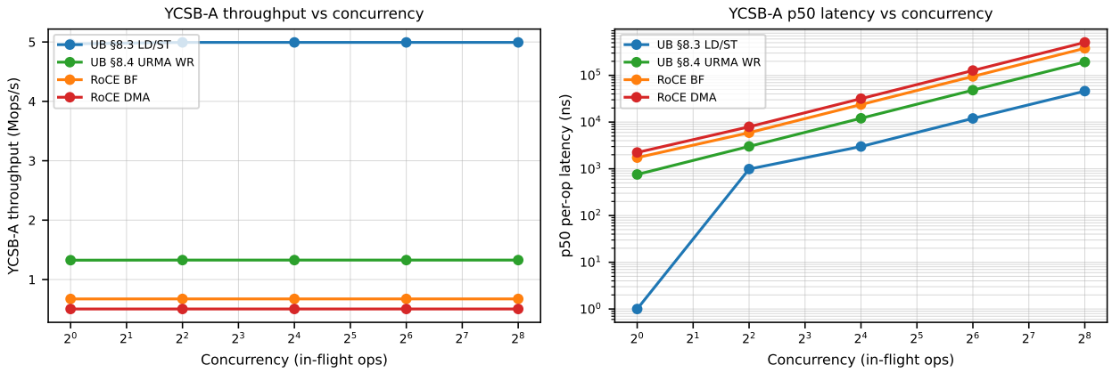
Figure 21: P3.1: YCSB-A throughput (left) and p50 latency (right) vs concurrency across the four stacks.
