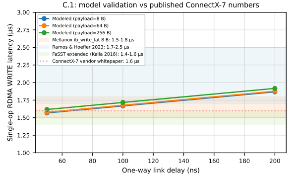
Figure 14: C.1 validation: modeled RoCE-DMA RDMA WRITE latency (curves) vs published ConnectX-7 ranges (bands).
