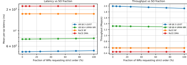
Figure 16: P2.1: latency (left) and throughput (right) vs SO fraction. UB scales linearly with mix; RoCE is flat (always-on strict order).
