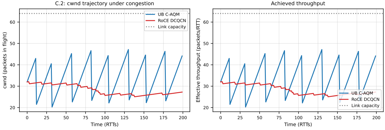
Figure 20: C.2: AIMD-modeled C-AQM vs DCQCN. cwnd trajectory and achieved throughput over 200 RTTs.
