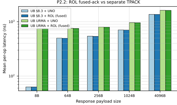
Figure 17: P2.2: ROL fused-ack vs separate TPACK. UB only.
