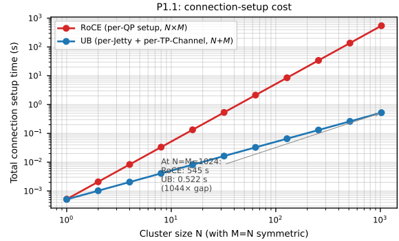
Figure 23: P1.1: total connection-setup time at symmetric N=M . RoCE's O(N \cdot M) vs UB's O(N+M) scaling.
