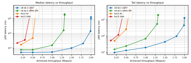
Figure 15: P3.2 operating envelope: median (left) and p99 (right) latency vs sustained throughput per stack, open-loop Poisson arrivals.
