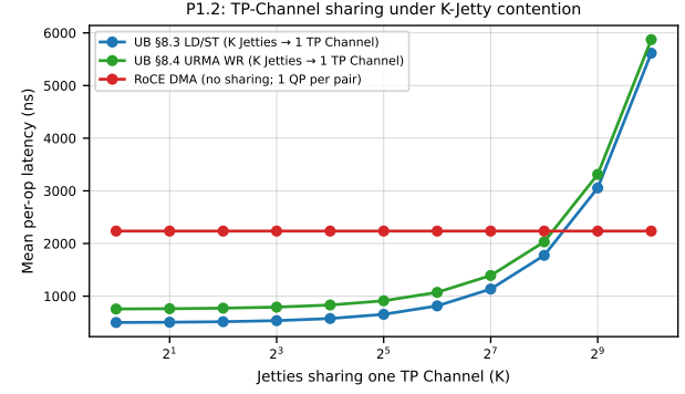
Figure 19: P1.2: UB per-op latency under K-Jetty contention. Linear PSN-allocator scaling; UB still wins until K \approx 255 .
