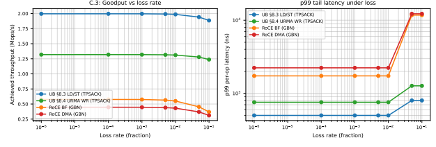
Figure 18: C.3: goodput (left) and p99 tail (right) vs loss rate. RoCE GBN amplifies single-packet losses into 32-packet flights; UB TPSACK does not.
