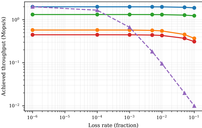
C.3: Goodput vs loss rate
