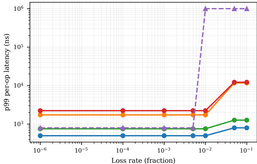
p99 tail latency under loss
