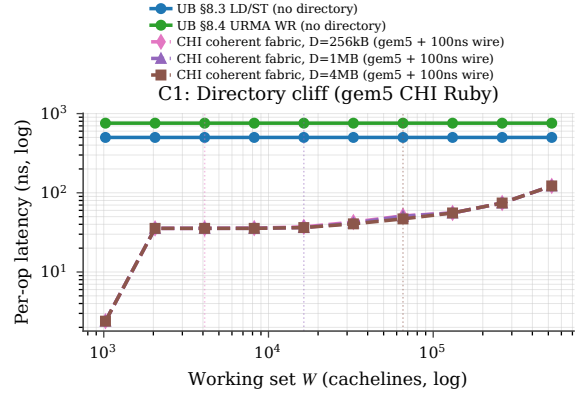
Figure 47: C1: per-op latency vs remote-cached working set W , measured on gem5 CHI Ruby with 100 ns intra-chassis wire delay. Three HNF/directory capacities are swept (256 kB, 1 MB, 4 MB); each curve accelerates sharply once W exceeds the directory size. UB’s two curves are constant in W .
