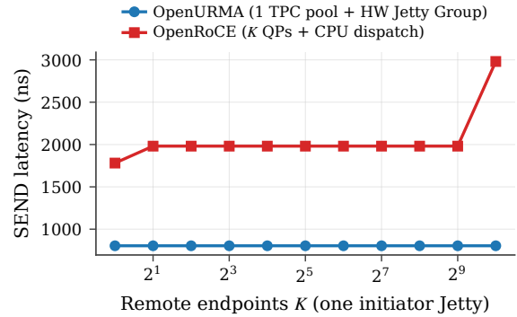
Figure 15: M2N fanout: one initiator Jetty addressing K remote endpoints. UB flat at 804 ns (one TPC pool + HW Jetty Group); RoCE jumps at K \geq 2 (CPU dispatch) and again at K = 1024 (NIC SRAM spill). SEND, 64 B, link 100 ns.
