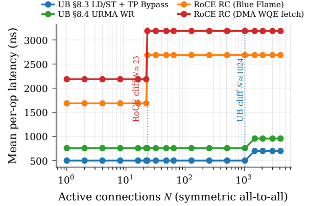
Figure 14: NIC SRAM context-cache spill. RoCE hits the cliff at N \approx 23 ( N^2 QPs > cache), adding \sim 1000 ns to every READ; UB hits it \sim 45\times later at N \approx 1024 , and its penalty is \sim 200 ns (membus, not PCIe).
