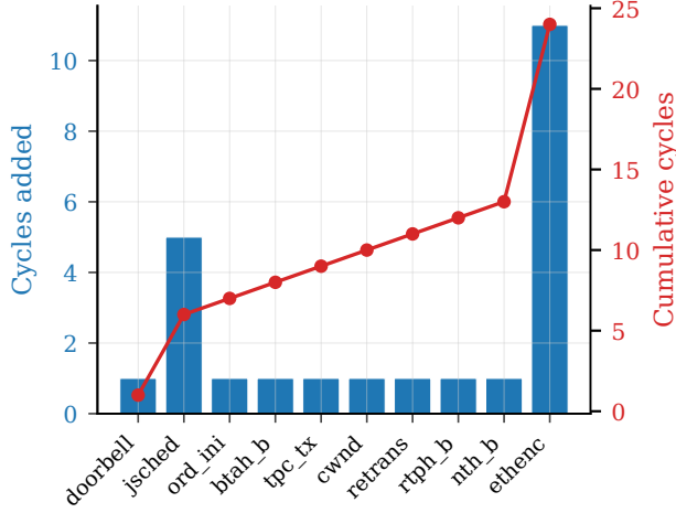
(a) Per-stage cycle cost (cumulative 24 cy at the wire).
