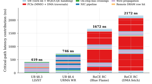
Figure 22: End-to-end latency budget by component, link = 100 ns, payload = 64 B, concurrency = 1.
