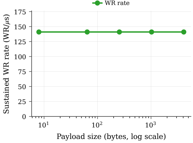
(b) Sustained WR rate vs payload — header-rate-limited.
