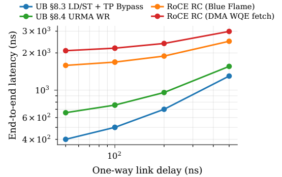
Figure 21: End-to-end latency vs one-way link delay on pointer-chase, concurrency = 1, payload = 64 B.
