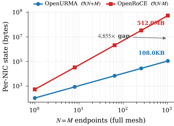
Figure 13: Per-NIC connection state vs endpoint count ( N=M ): OpenURMA’s O(N+M) vs RoCE’s O(N \cdot M) , reaching 4,855\times at 1024 endpoints.
