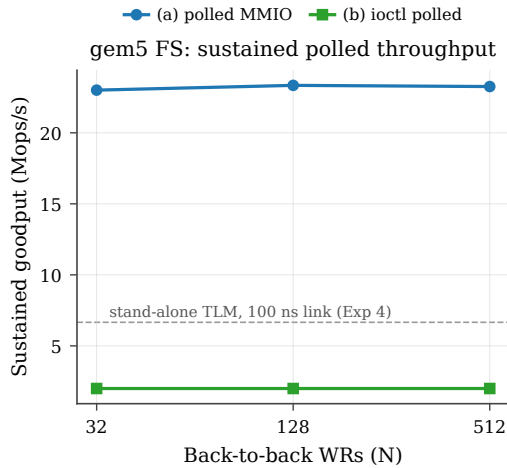
Figure 32: gem5 FS-mode sustained polled goodput vs back-to-back WR count. The polled-MMIO path (a) holds \sim 23 Mops/s; the ioctl path (b) holds \sim 2 Mops/s. Dashed line marks the stand-alone-TLM 6.66 Mops/s envelope (link-limited); gem5's self-loop has zero link delay so the SC pipeline is the bottleneck, not the wire.
