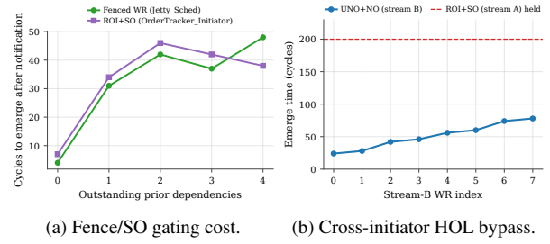
Figure 34: Ordering cost in isolation. (a) Cycles from completion notification to a gated WR’s emission (Fence, SO), both under 50. (b) UNO+NO WRs from four initiators emerge while a separate initiator’s ROI+SO is held indefinitely — no back-pressure.
