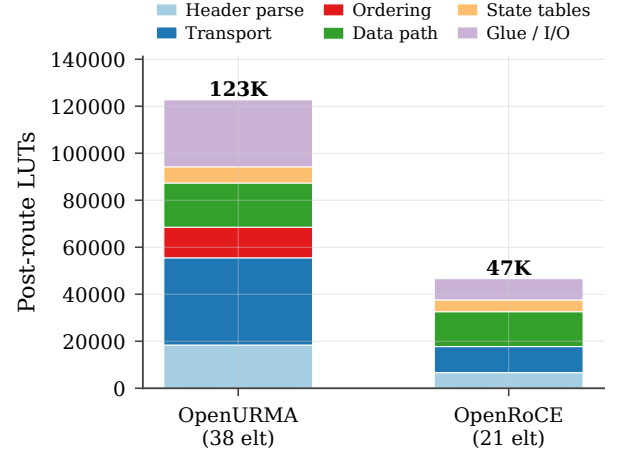
Figure 9: Post-route LUT budget by architectural role for both stacks.
