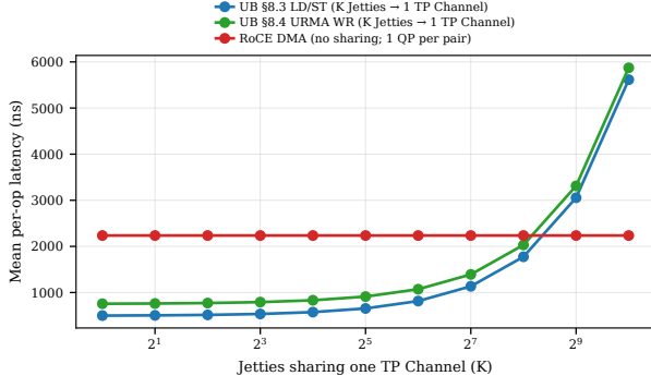
Figure 16: Per-op latency under K -Jetty contention on one TP Channel. Linear PSN allocator scaling; UB beats per-QP RoCE until K \approx 255 .
