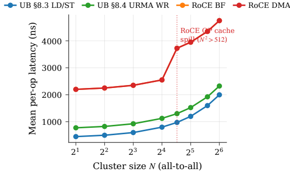
Figure 17: Cluster-scale per-op latency vs node count. RoCE crosses the QP-cache spill at N=23 ; UB stays bounded.
