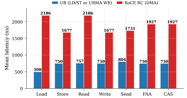
Figure 23: Per-verb mean latency comparison. UB (§8.3 LD/ST for Load/Store; §8.4 URMA WR for Read/Write/Send; §7.4.2.3 atomics for FAA/CAS) vs RoCE RC (DMA WQE fetch). Link = 100 ns, concurrency = 1, payload = 64 B (atomics: 8 B operand).
