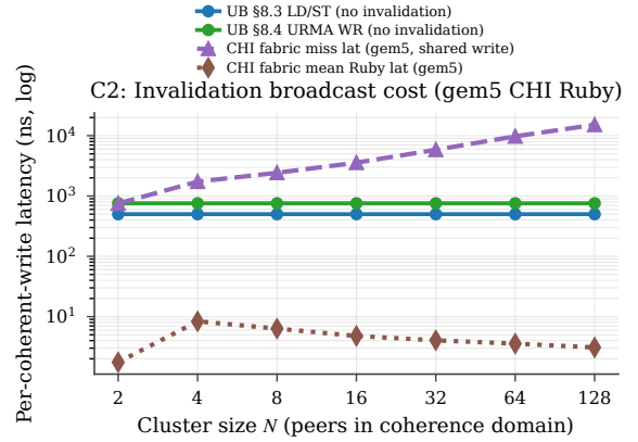
Figure 48: C2: per-coherent-write latency vs cluster size N , measured on gem5 CHI Ruby with 100 ns intra-chassis wire and shared-process pthread workload. CHI miss latency grows from 750 ns at N=2 to 15170 ns at N=128 ( \sim N^{0.65} ), while UB stays flat at 500 ns.
