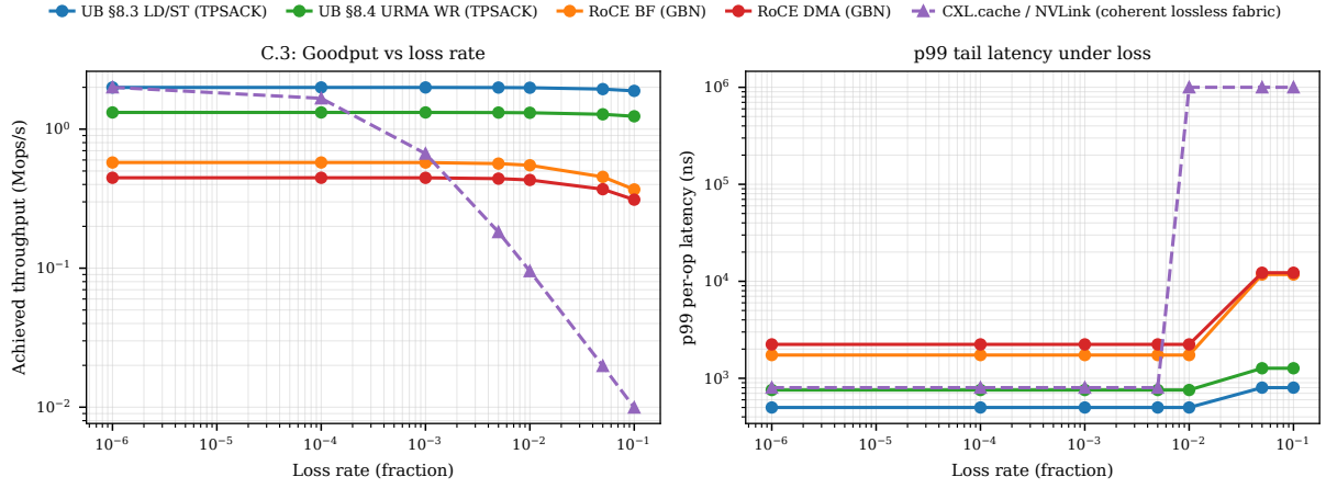
Figure 44: Goodput (left) and p99 tail (right) vs loss rate. Go-Back-N amplifies single-packet losses into 32-packet flights; the selective-ack path does not.
