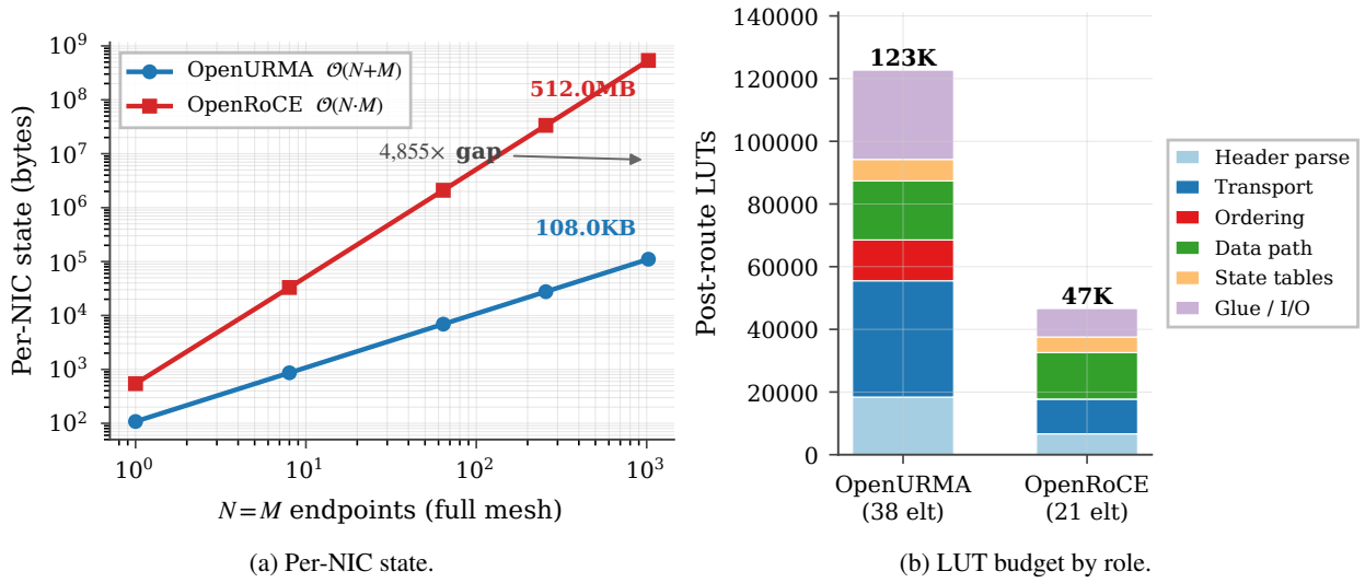
Figure 32: (a) State scaling over (N=M) for OpenURMA’s \mathcal{O}(N+M) design vs RoCE’s \mathcal{O}(N \cdot M) ; 4,855 \times at 1024 endpoints. (b) Post-route LUT budget by architectural role for both stacks.
