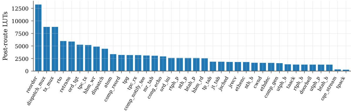
Figure 31: Per-element post-route LUT, sorted descending. All 38 OpenURMA elements meet 322 MHz with positive WNS. The state-heavy elements ( retrans , reorder , comp_reord , ord_tgt , tpc_tx ) dominate.
