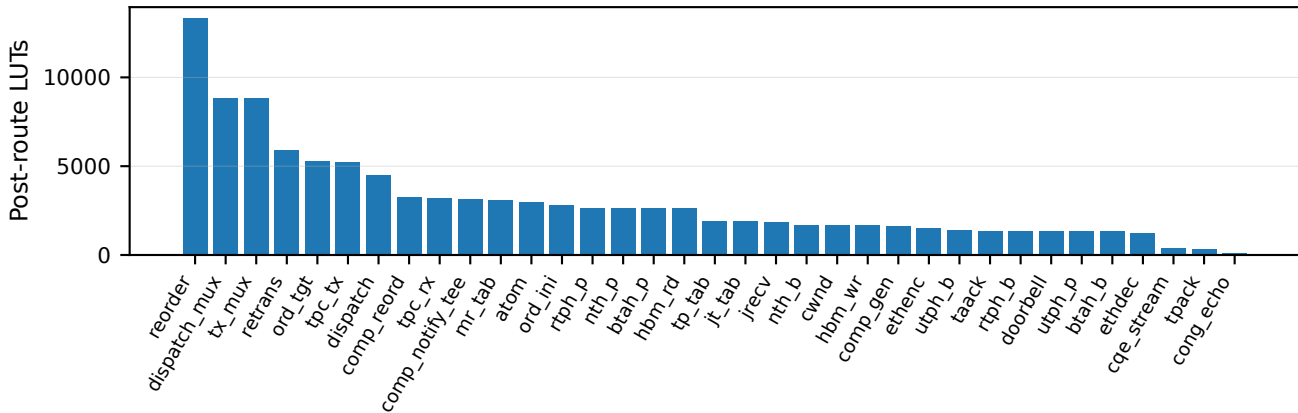
OpenURMA per-element LUT (sorted; all elements meet 322 MHz)
