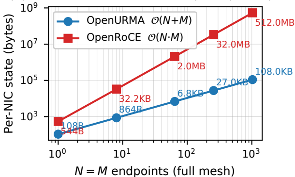
(a) Per-NIC state scales as \mathcal{O}(N+M) vs \mathcal{O}(N \cdot M)
