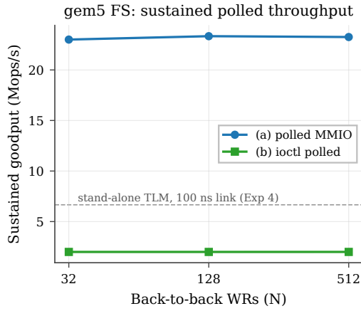
Figure 27: gem5 FS-mode sustained polled goodput vs back-to-back WR count. The polled-MMIO path (a) holds \sim 23 Mops/s; the ioctl path (b) holds \sim 2 Mops/s. Dashed line marks the standalone-TLM 6.66 Mops/s envelope (link-limited); gem5’s self-loop has zero link delay so the SC pipeline is the bottleneck, not the wire.
