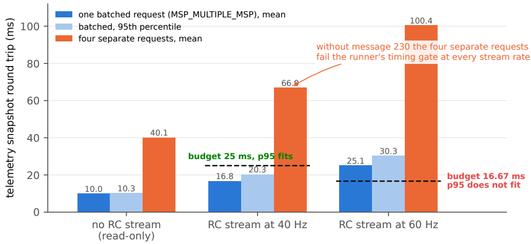
Figure 21: One 115200-baud UART carries both the telemetry and the stick stream. Telemetry snapshot latency (attitude, raw IMU, status and RC in one round trip) with and without the stick stream, batched against the four-request fallback; 300 samples per condition, measured on the aircraft over USB on 21 September.
