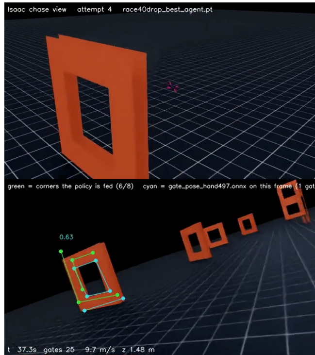
Figure 20: The race40drop policy racing in Isaac under the measured corner dropout, gates 22 to 29 of a run that passed 38 gates in 58 s from the pad ( race40drop_pov.mp4 , real time; the GIF is ten seconds of it). Above: the chase view. Below: the drone's own camera, with the target gate's corners drawn in green exactly as the policy was fed them that step, latch, delay and dropout included, and in cyan every gate the real hand497 detector finds on the same rendered frame with its box confidence. The detector was trained on photographs of real gates and never on renders, and it fires on Isaac's orange squares on most frames, usually on the gate the policy is flying at and often on the ones behind it.
