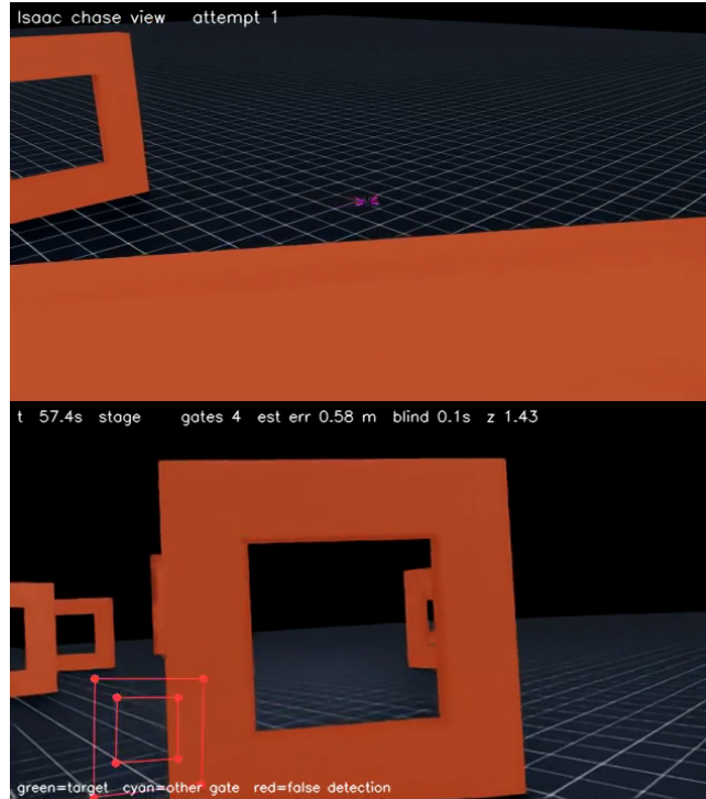
Figure 25: Ten seconds of the classical stack flying in Isaac ( stack_pov.mp4 , real time, 127 s): staging in front of gate 4, settling, passing it and turning to gate 5. The full run reached nine of the ten gates before losing its position estimate. Above: Isaac’s chase view. Below: the drone’s own camera with the simulated detector’s corners drawn, green for the target gate, cyan for other gates, red for false detections, and a status line of time, phase, gates passed, estimation error and time blind. Three earlier attempts, side by side at twice real time, are stack_run_01 , 02 and 03 .
