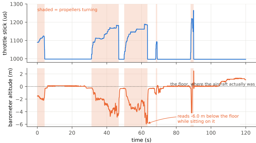
Figure 22: Aircraft armed on the ground, 18 September: throttle stick and barometric altitude over two minutes of MSP telemetry at 23.6 Hz, with the intervals when the propellers were turning shaded. Each throttle rise reads as a descent of several metres, which is why every hover design took height from the camera.
