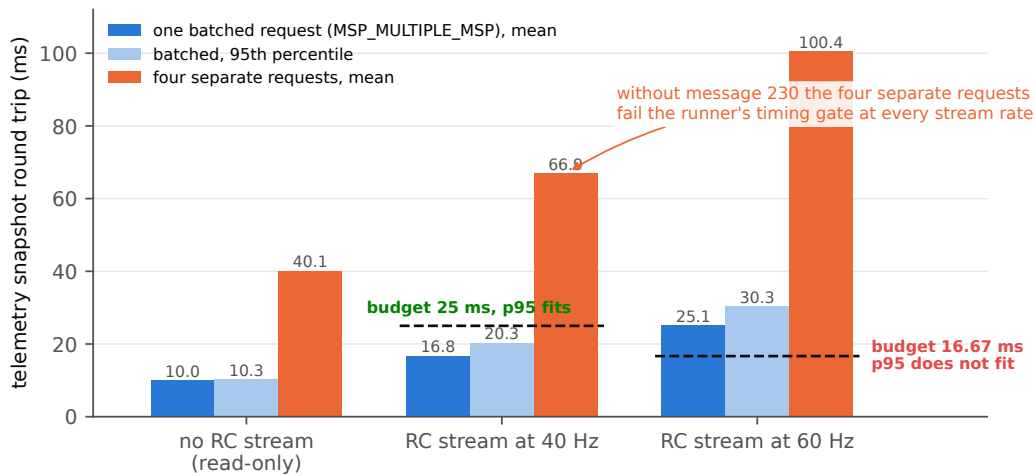
Figure 20: One 115200-baud UART carries both the telemetry and the stick stream. Telemetry snapshot latency (attitude, raw IMU, status and RC in one round trip) with and without the stick stream, batched against the four-request fallback; 300 samples per condition, measured on the aircraft over USB on 21 September.
