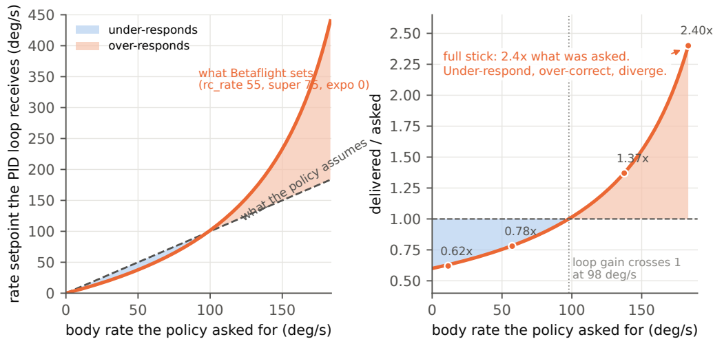
Figure 21: The shipped linear stick map against the flight controller's rate curve. The policy's 3.2 rad/s (183°/s) envelope was sent to full stick, where this profile (rc_rate 55, super rate 75, expo 0, read off the aircraft) commands 440°/s. Every runner on this stack validated commands to the same envelope, so the finding applied to every policy, not one.
