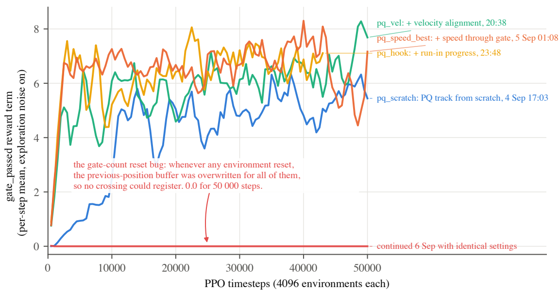
Figure 11. The lineage that produced pq_speed_best , from the surviving TensorBoard logs: each run on the team's PQ track warm-started from the one before it, 4–5 September, and the continuation on 6 September with identical settings that passed no gates. The continuation was the first symptom of a reset bug: whenever any environment reset, the previous-position buffer was overwritten for all environments, so no crossing could ever be registered again. A one-line fix confirmed by an A/B test restored the gate reward from 0.01 to 1.1.
