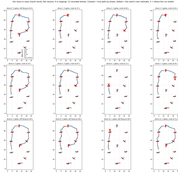
Figure 24: The classical fallback stack flown in Isaac against the pessimistic sensor model: twelve attempts from the pad in plan view, true path in blue, the stack's own position estimate dotted, a cross where the run ended. Most crashes fall between gates 5 and 6, where the course reverses.
