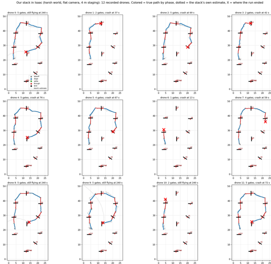
Figure 23. The classical fallback stack, flown in Isaac against a pessimistic sensor model (every gate detected, gate-shaped false positives, sticky corner dropout, 60 ms latency, an unknown self-levelling gain). Most crashes fall between gates 5 and 6, where the course reverses.
