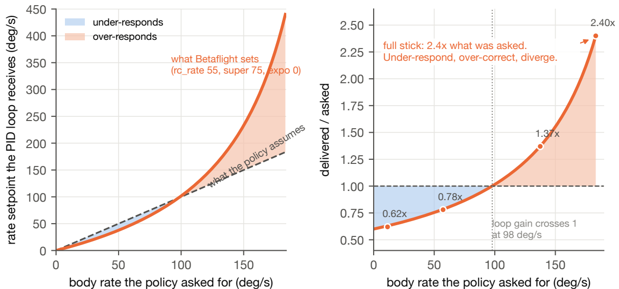
Figure 21. The shipped linear stick map against the flight controller's rate curve. The policy's 3.2 rad/s ( 183^\circ/\text{s} ) envelope was sent to full stick, where this profile (rc_rate 55, super rate 75, expo 0, read off the aircraft) commands 440^\circ/\text{s} . Every runner on this stack validated commands to the same envelope, so the finding applied to every policy, not one.
