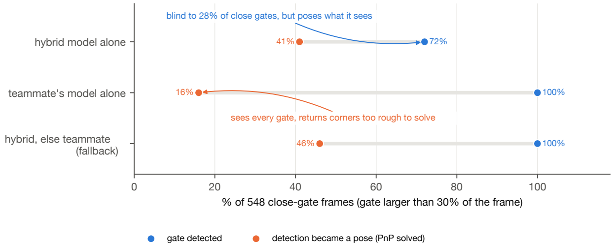
Figure 8. Close gates are the ones flown through, and the two models fail in opposite directions. On the 548 close-gate frames of the walk-around capture (laptop CPU, 640×360): blue is the gate being found, orange is its corners being good enough for a pose. The hybrid model is near-blind to 28% of close gates but poses what it sees; the teammate’s model sees every gate and returns corners too rough to solve; the combination beats both.
