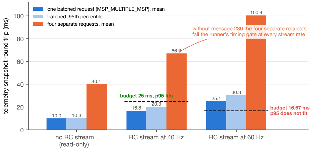
Figure 20. One 115200-baud UART carries both the telemetry and the stick stream. Telemetry snapshot latency (attitude, raw IMU, status and RC in one round trip) with and without the stick stream, batched against the four-request fallback; 300 samples per condition, measured on the aircraft over USB on 21 September.
