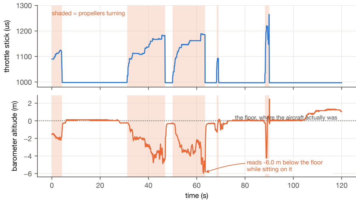
Figure 22. Aircraft armed on the ground, 18 September: throttle stick and barometric altitude over two minutes of MSP telemetry at 23.6 Hz, with the intervals when the propellers were turning shaded. Each throttle rise reads as a descent of several metres, which is why every hover design took height from the camera.
