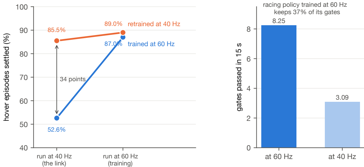
Figure 15. The control rate is part of the plant. Left: hover settled fraction for the 60 Hz checkpoint and the 40 Hz retrain, each run at both rates (4096 episodes). Right: the 60 Hz racing checkpoint's gates in 15 s at both rates.
