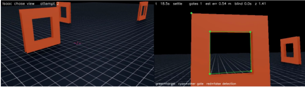
Figure 25: Ten seconds of the classical stack flying in Isaac ( stack_run_02.mp4 , 60 s; runs 01 and 03 are the other two attempts). Left: Isaac’s chase view. Right: the drone’s own camera with the simulated detector’s corners drawn, green for the target gate, cyan for other gates, red for false detections, and a status line of time, phase, gates passed, estimation error and time blind.
