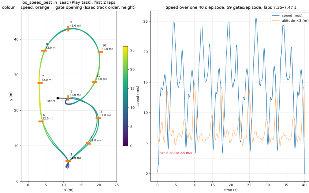
Figure 10: pq_speed_best in playback on the team’s original track: path over two laps coloured by speed, and speed and altitude against time. The dashed line is the fallback plan’s 2.5 m/s gate speed for comparison.
