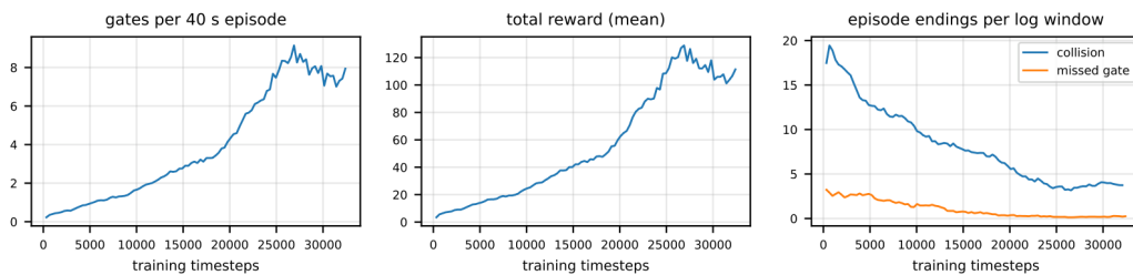
Figure 14: Training curves of the one-hour fine-tune on the corrected simulator: gates per 40 s episode, mean total reward, and episode endings by cause.
