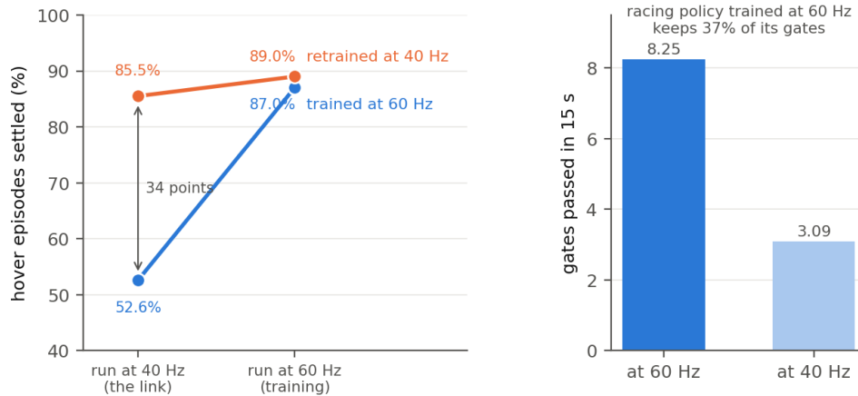
Figure 15: The control rate is part of the plant. Left: hover settled fraction for the 60 Hz checkpoint and the 40 Hz retrain, each run at both rates. Right: the 60 Hz racing checkpoint's gates in 15 s at both rates.
