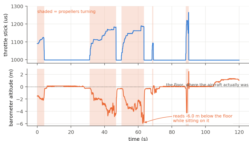
Figure 22: Throttle stick and barometric altitude over two minutes with the aircraft armed on the ground. Each throttle rise reads as a descent of several metres.
