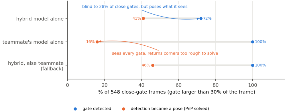
Figure 8: On the 548 close-gate frames of the walk-around capture (laptop CPU, 640×360): the hybrid model is near-blind to 28% of close gates but poses what it sees; the teammate’s model sees every gate and returns corners too rough to solve; the combination beats both.
