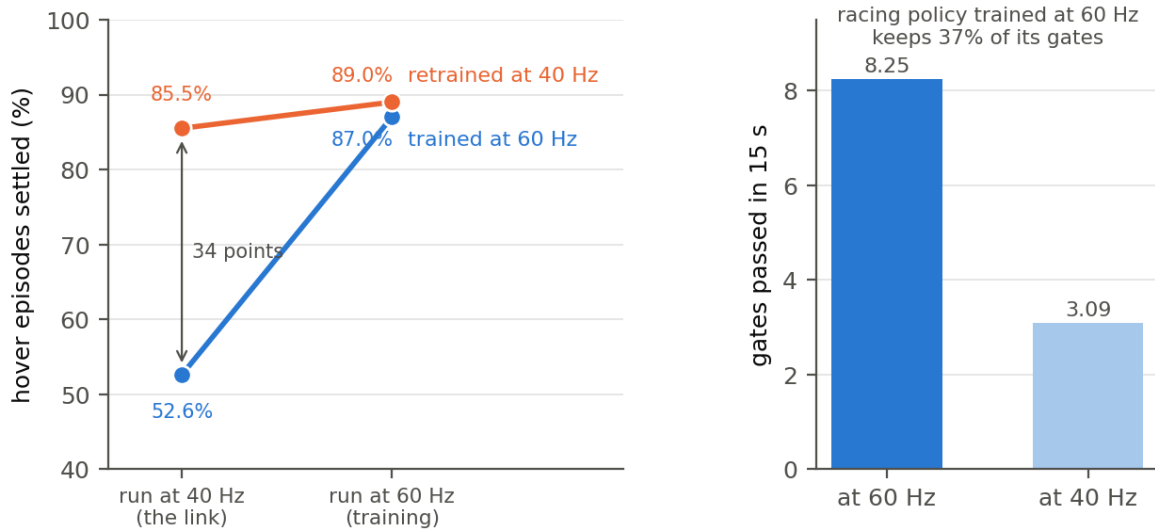
Figure 15. The control rate is part of the plant. Left: hover settled fraction for the 60 Hz checkpoint and the 40 Hz retrain, each run at both rates. Right: the 60 Hz racing checkpoint's gates in 15 s at both rates.
