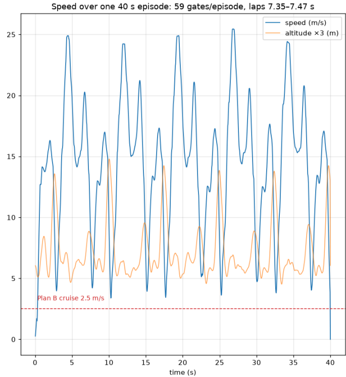
Figure 10. pq_speed_best in playback on the team's original track: path over two laps coloured by speed, and speed and altitude against time. The dashed line is the fallback plan's 2.5 m/s gate speed for comparison.
