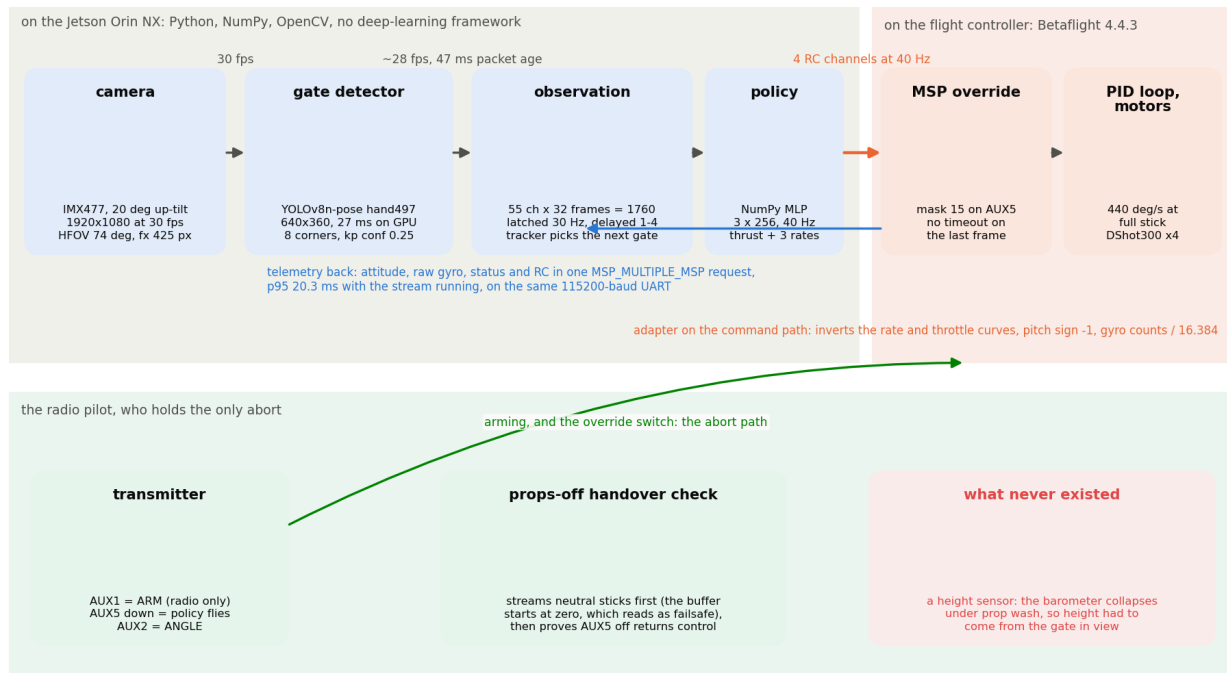
Figure 3. The chain from photons to motors as it stood on 21 September, with the rate or latency measured on each link. The lower band is the part of the system the pilot owns: arming and the override switch are the only abort, and the props-off handover check is the test that proves they work. The box on the right is the sensor the aircraft never had.
