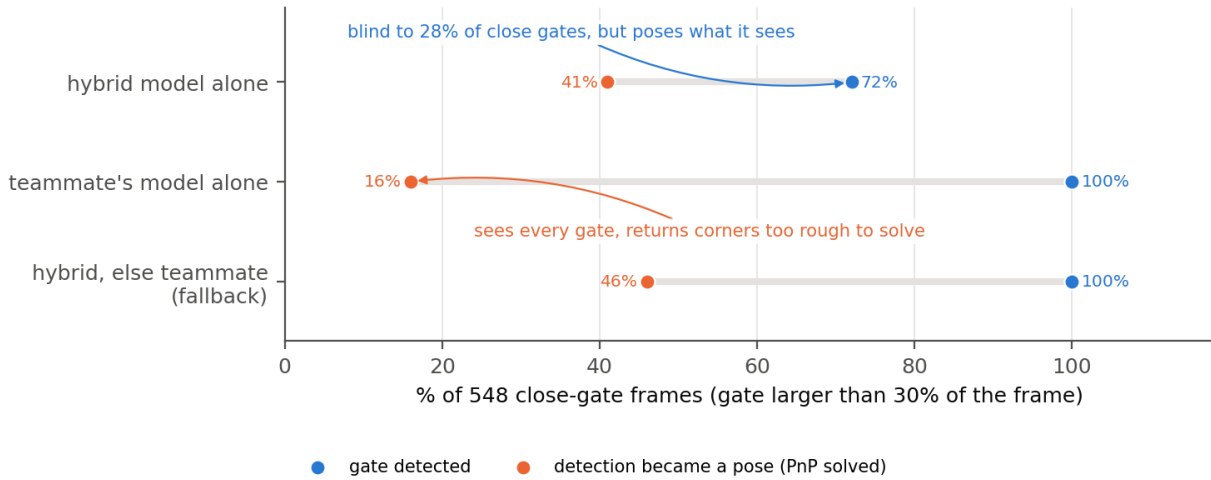
Figure 8. On the 548 close-gate frames of the walk-around capture (laptop CPU, 640x360): the hybrid model is near-blind to 28% of close gates but poses what it sees; the teammate’s model sees every gate and returns corners too rough to solve; the combination beats both.
