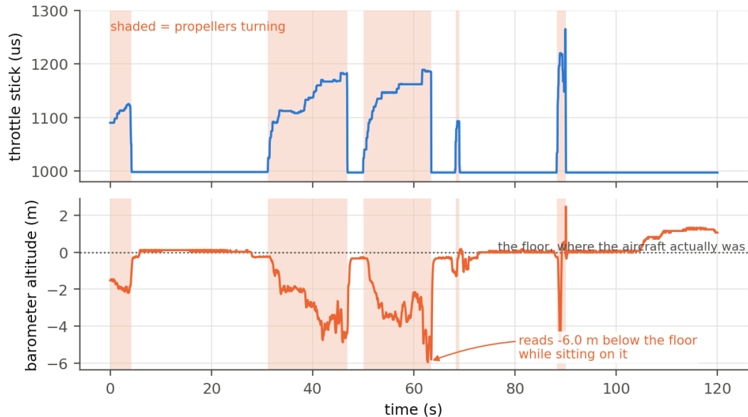
Figure 22. Throttle stick and barometric altitude over two minutes with the aircraft armed on the ground. Each throttle rise reads as a descent of several metres.
