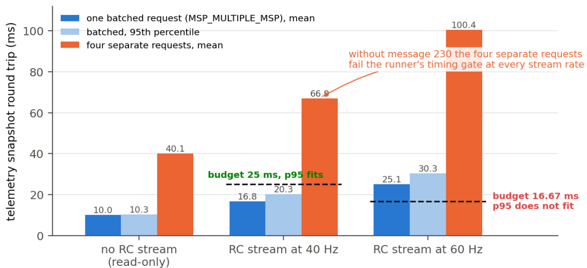
Figure 20. Telemetry snapshot latency with and without the stick stream, batched against the four-request fallback. 300 samples per condition, measured on the aircraft over USB.
