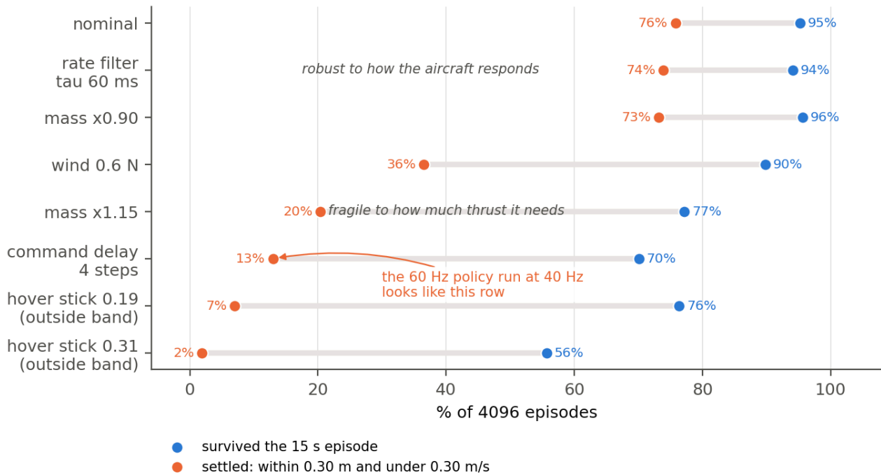
Figure 16. The hover policy under eight perturbations, 4096 episodes each. The hover-stick rows are outside the trained band and outside what the aircraft does; they bound the failure mode rather than describe a live risk.
