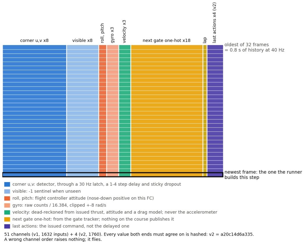
Figure 9. The observation as the policy receives it: one row per frame, thirty-two frames deep, one column per channel, coloured by where the channel comes from. The bottom row is the frame the runner builds this step; everything above it is history.
