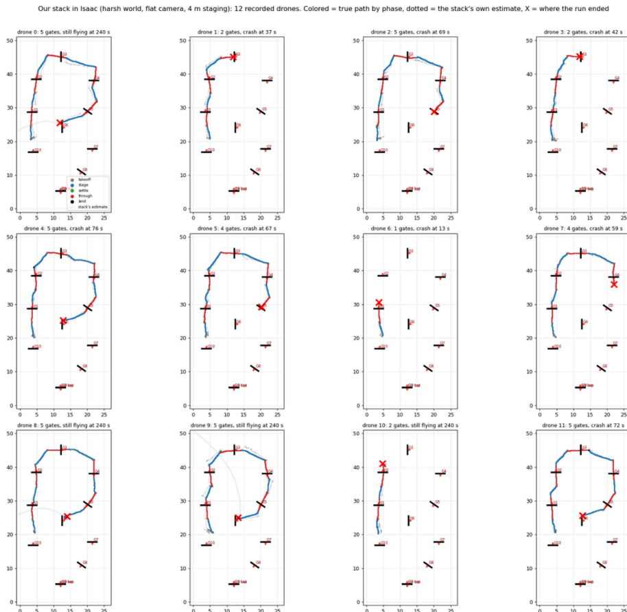
Figure 23. The classical fallback stack, flown in Isaac against a pessimistic sensor model (every gate detected, gate-shaped false positives, sticky corner dropout, 60 ms latency, an unknown self-levelling gain). Most crashes fall between gates 5 and 6, where the course reverses.
