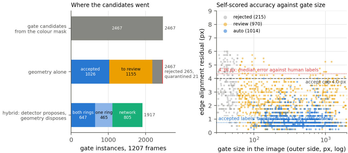
Figure 6. The auto-labeller's 2467 gate candidates from the walk-around capture and where each went, then the hybrid's yield; right, every candidate's edge-alignment residual against its size in the image. The blue median is the labeller scoring itself; the red line is what human labels later measured. The gap between them is the systematic error the self-score cannot see.
