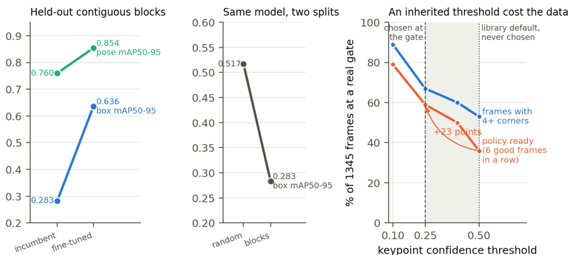
Figure 5. Left: the teammate's model against the fine-tune, on held-out contiguous blocks. Centre: the same model scored two ways. Right: the keypoint confidence threshold the runner inherited from the library (0.5) against the value chosen at a real gate (0.25), measured over 1345 frames; the gate itself was detected in every frame at every setting.
