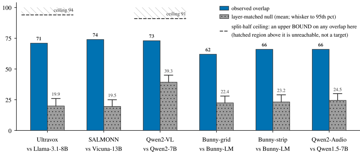
top-100 head overlap (of 100)
