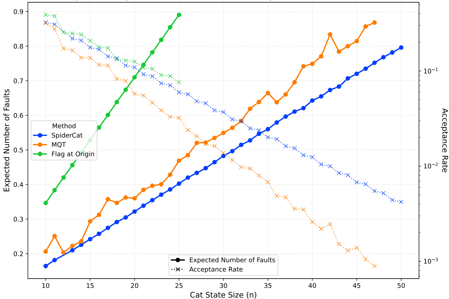
Method Comparison: Expected Number of Faults & Acceptance Rate vs CAT state size (t=5)
