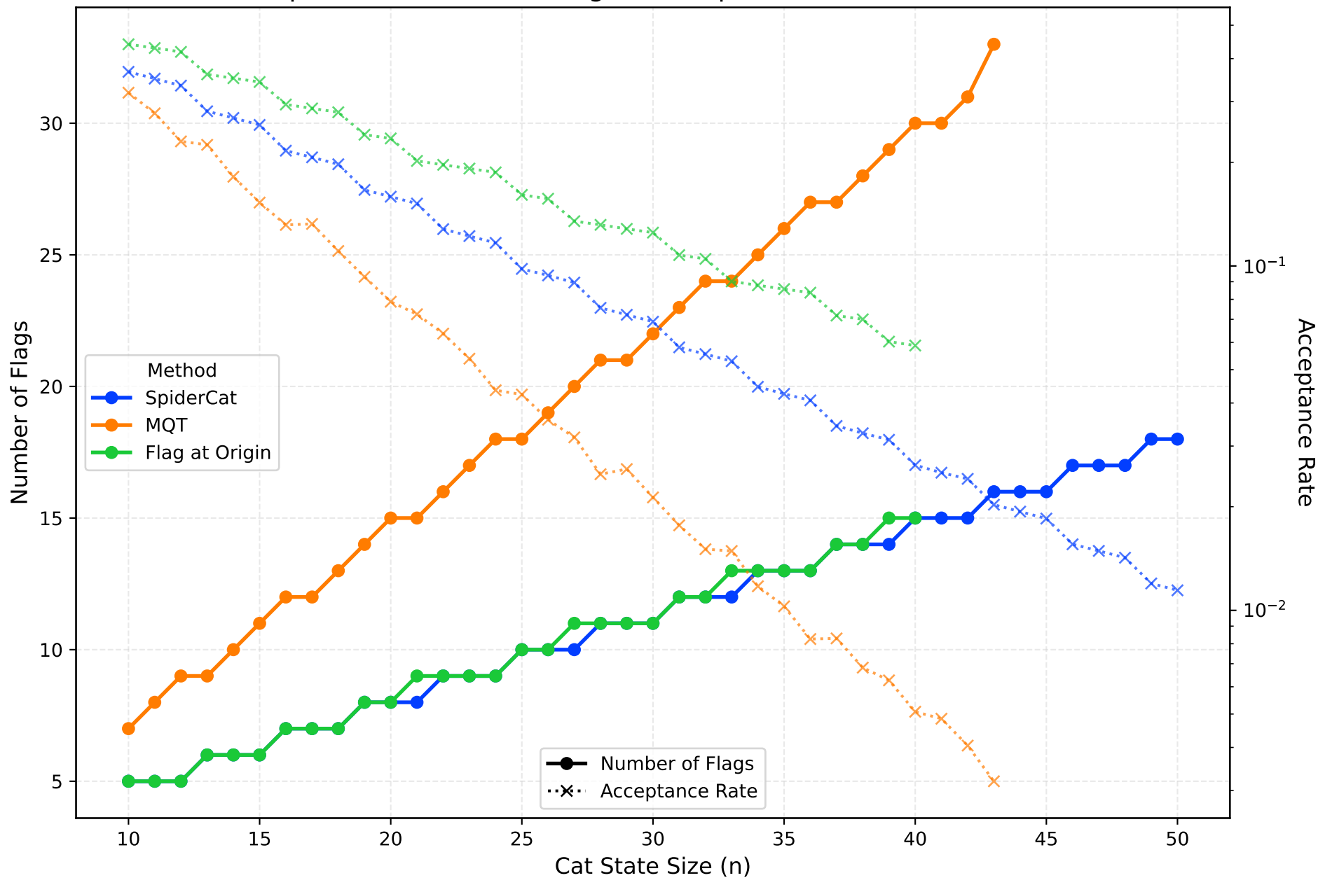
Method Comparison: Number of Flags & Acceptance Rate vs CAT state size (t=3)
