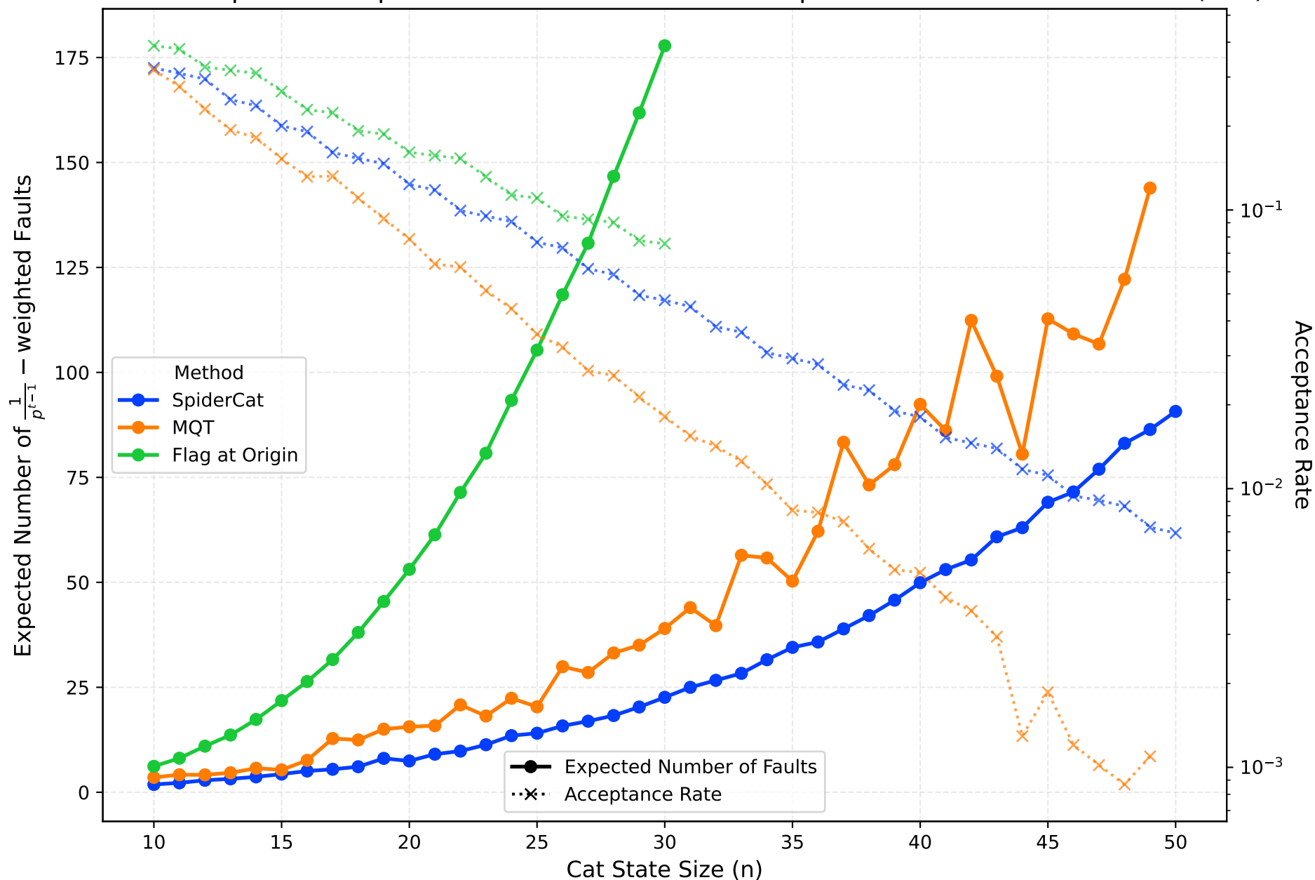
Method Comparison: Expected Number of Faults & Acceptance Rate vs CAT state size (t=4)
