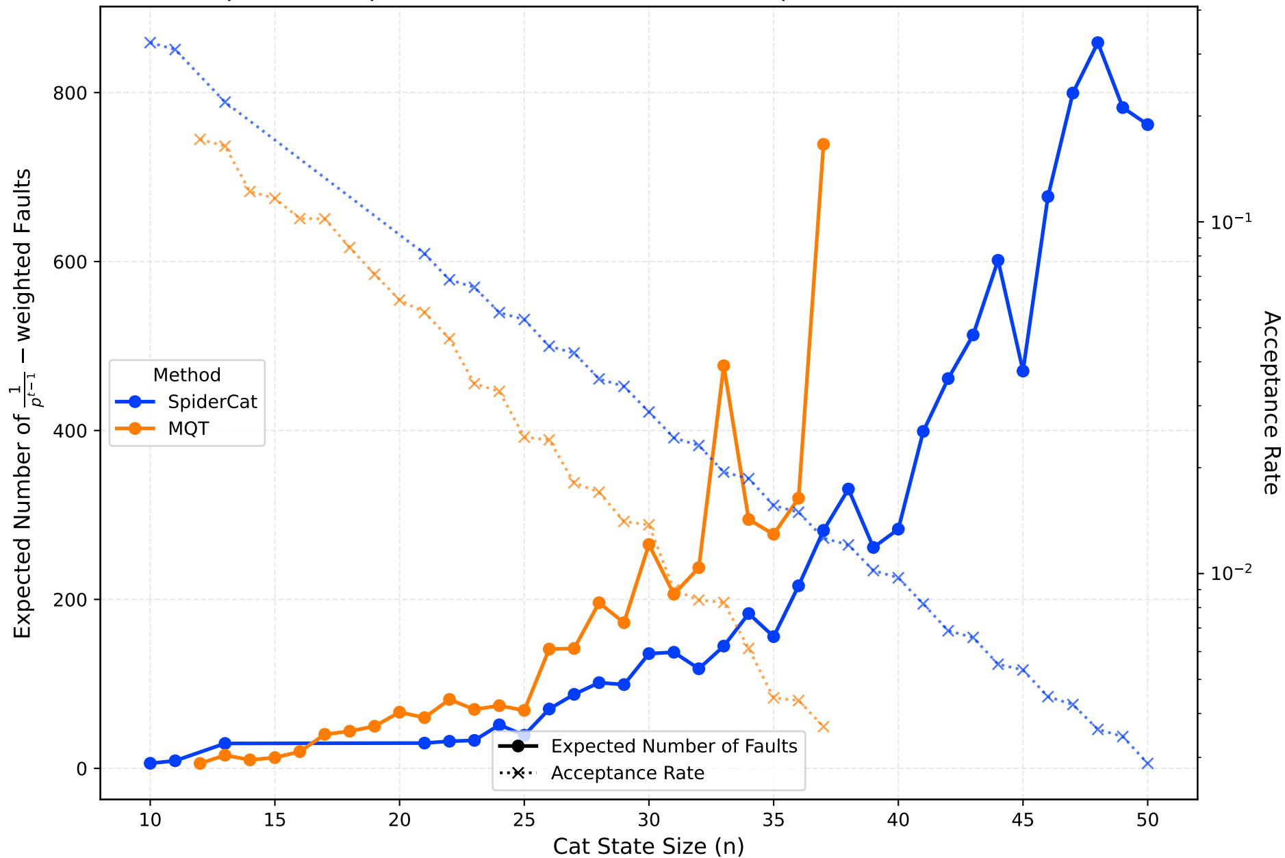
Method Comparison: Expected Number of Faults & Acceptance Rate vs CAT state size (t=6)
